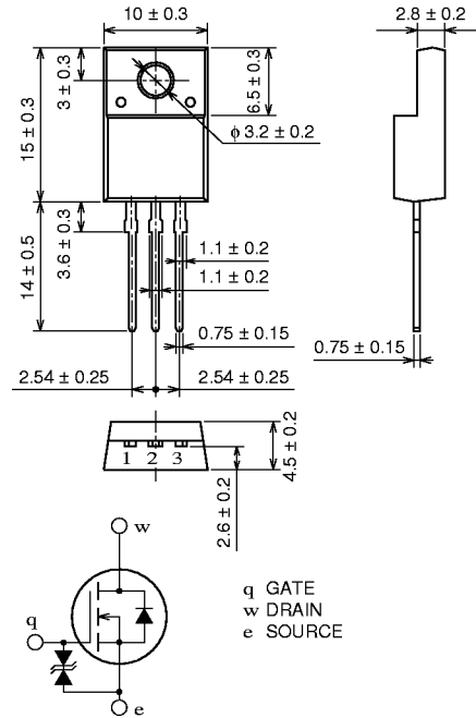
TO-220FN
