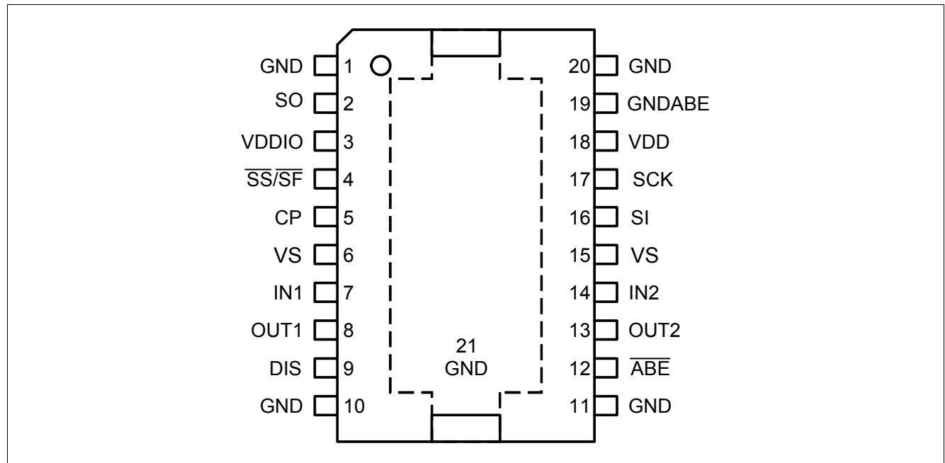
Figure 1 Pinout TLE8209-4SA
