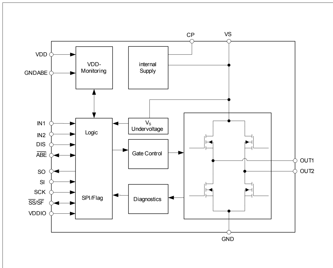
Figure 3 Block Diagram TLE8209-4SA
