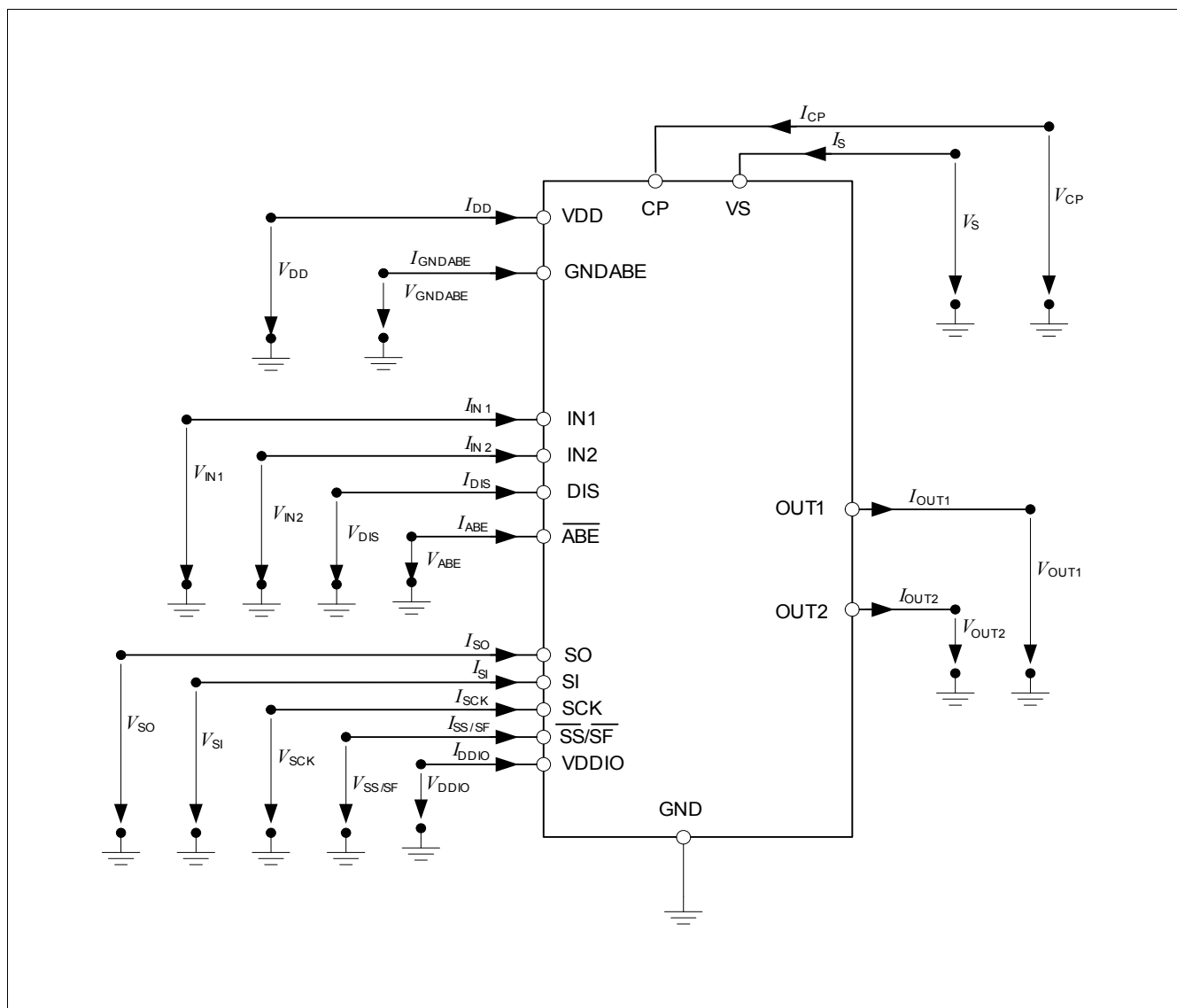
Figure 2 Terms TLE8209-4SA
