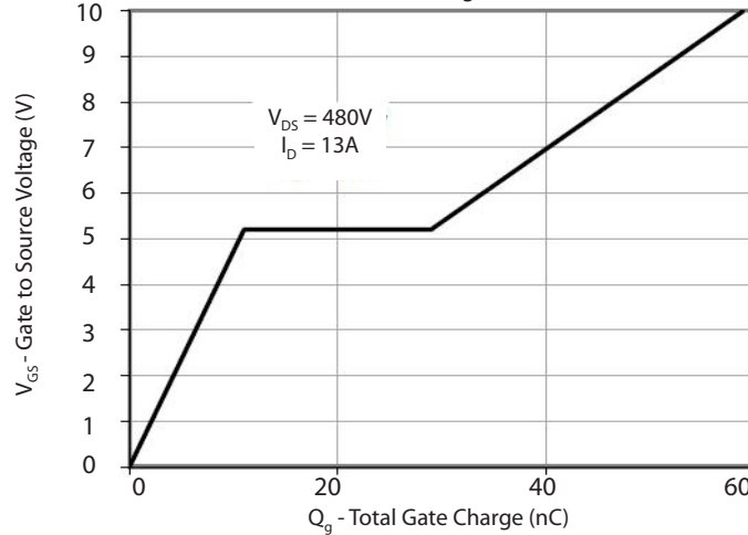
Gate Charge
