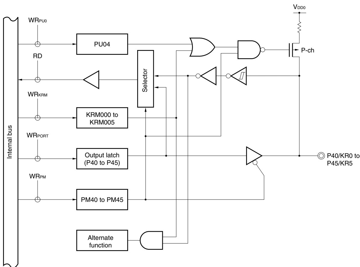
Figure 4-8. Block Diagram of P40 to P45
