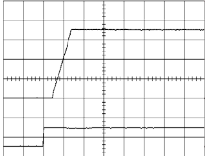
Start-up enabled by connecting V_I at: T_{ref} = +25^\circ\text{C} , I_O = 15\text{ A} resistive load, V_I = 5.0\text{ V} . Top trace: output voltage (0.5 V/div.). Bottom trace: input voltage (5 V/div.). Time scale: 5 ms/div..
