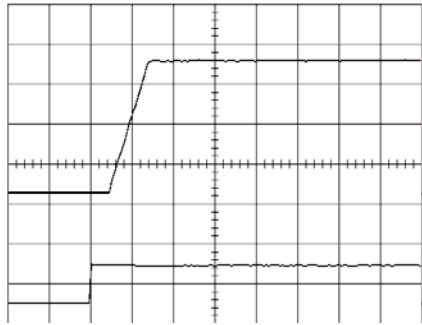
Start-up enabled by connecting V_i at: T_{ref} = +25^{\circ}\text{C} , I_O = 15\text{ A} resistive load, V_i = 5.0\text{ V} . Top trace: output voltage (1.0 V/div.). Bottom trace: input voltage (5 V/div.). Time scale: 5 ms/div..
