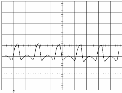
Output voltage ripple (20mV/div.) at: T_{ref} = +25^\circ\text{C} , I_O = 15\text{ A} resistive load, V_i = 5.0\text{ V} . Time scale: 2 \mu\text{s}/\text{div} . See the filter in the Output ripple and noise section (EMC Specification).
