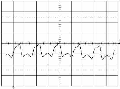
Output voltage ripple (20mV/div.) at: T_{ref} = +25^\circ\text{C} , I_O = 15\text{ A} resistive load, V_I = 5.0\text{ V} . Time scale: 2 μs/div. See the filter in the Output ripple and noise section (EMC Specification).
