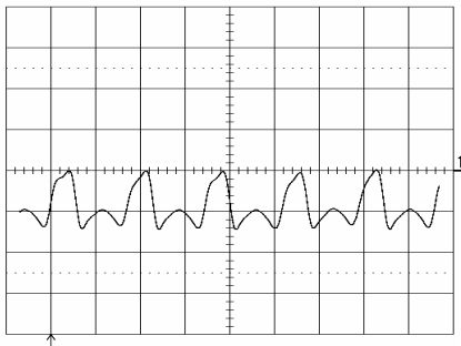
Output voltage ripple (20mV/div.) at: T_{ref} = +25^\circ\text{C} , I_o = 15\text{ A} resistive load, V_i = 5.0\text{ V} . Time scale: 2 \mu\text{s}/\text{div} . See the filter in the Output ripple and noise section (EMC Specification).
