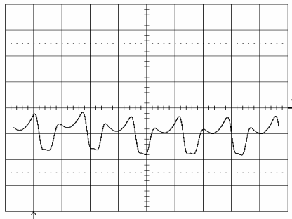
Output voltage ripple (20mV/div.) at: T_{ref} = +25^{\circ}\text{C} , I_O = 15\text{ A} resistive load, V_i = 5.0\text{ V} . Time scale: 2 \mu\text{s}/\text{div} . See the filter in the Output ripple and noise section (EMC Specification).
