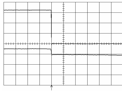
Shut-down enabled by disconnecting V_i at: T_{ref} = +25^{\circ}\text{C} , I_O = 15\text{ A} resistive load, V_i = 5.0\text{ V} . Top trace: output voltage (1.0 V/div.). Bottom trace: input voltage (2 V/div.). Time scale: 5.0 ms/div..
