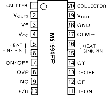
Outline 20P2N
