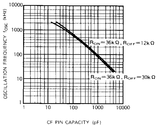
OSCILLATION FREQUENCY VS. CF PIN CAPACITY
