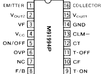
Outline 16P4
