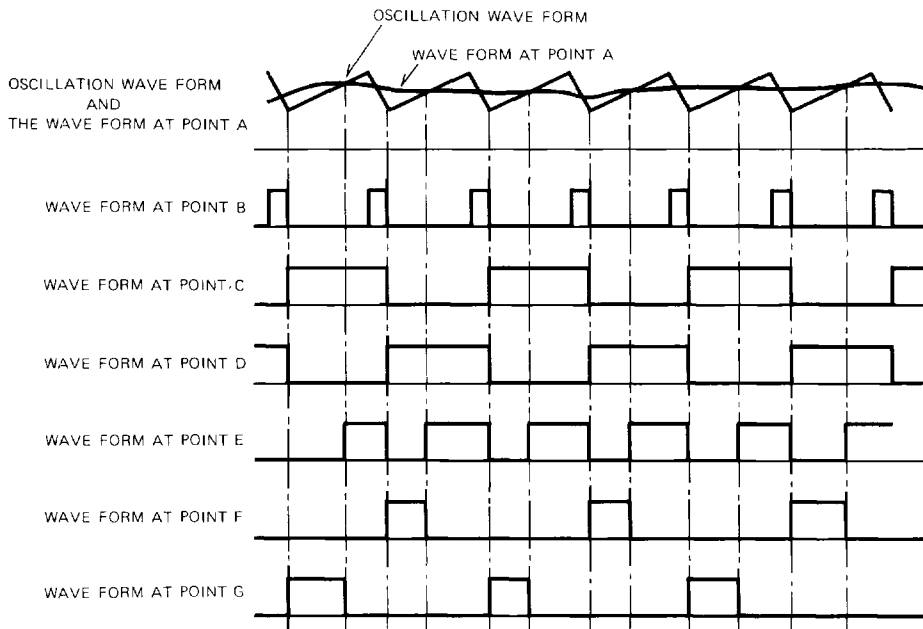
Figure 6 Wave forms at each point of the PWM comparator and the steering circuit
