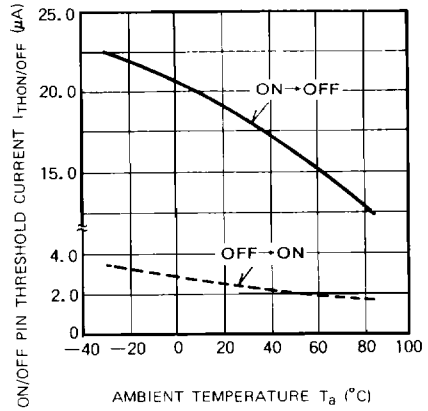
ON/OFF PIN THRESHOLD CURRENT VS. AMBIENT TEMPERATURE
