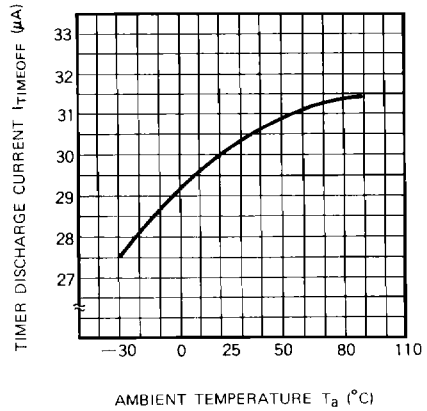
TIMER DISCHARGE CURRENT VS. AMBIENT TEMPERATURE
