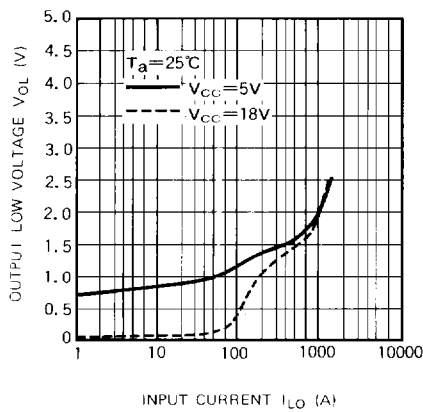
OUTPUT LOW VOLTAGE VS. INPUT CURRENT
