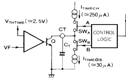
Figure 10 Block diagram of intermittent circuit
