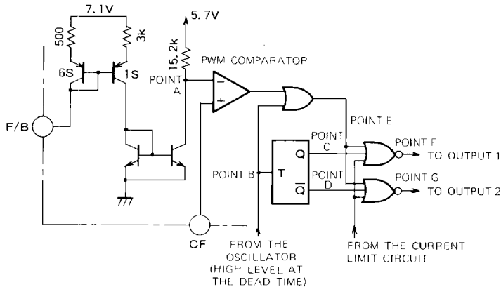
Figure 5 PWM comparator and steering circuit sections
