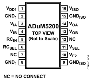
Figure 6. ADuM5200 Pin Configuration
