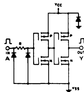
SCL4050B
