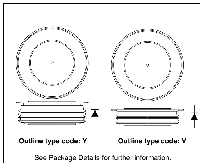
Fig. 1 Package outlines
