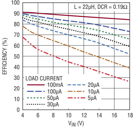
Buck Efficiency vs V_{IN} , for V_{IN} = 3.3\text{V}
