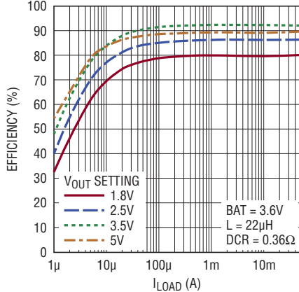
Buck-Boost Efficiency vs I_{LOAD} , 250mA Setting
