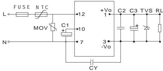
Figure 1: LS03-05BXXK can use MORNSUN's FC-L01D
