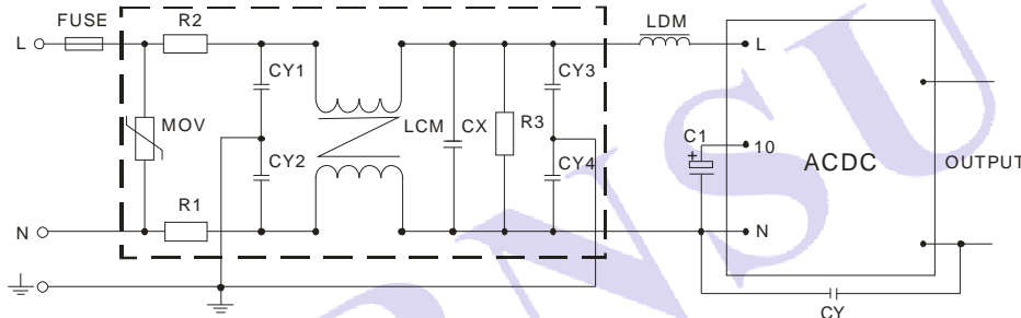
Figure 3: LS03 series Recommended circuit for application require higher EMC standard (external circuit output same as above)
