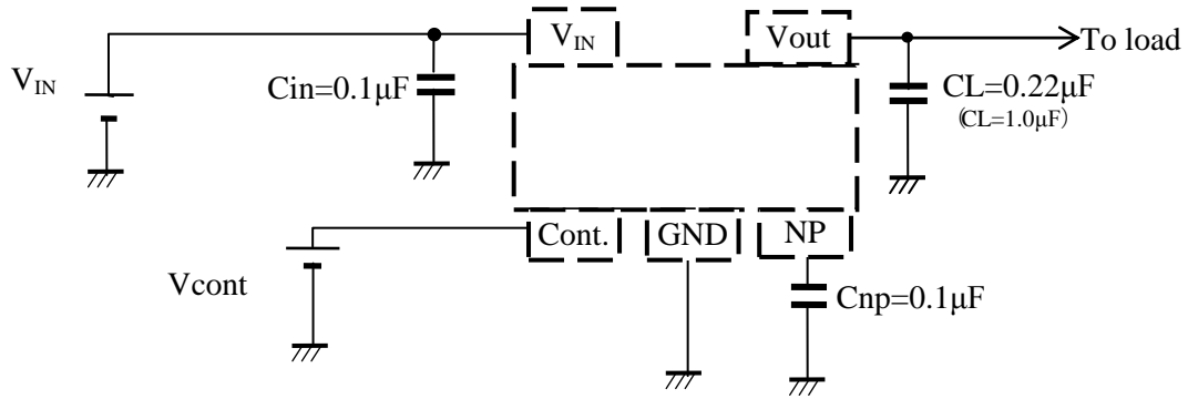
Figure 7. External Circuit
