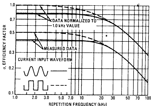
FIGURE 15 – RECTIFICATION WAVEFORM EFFICIENCY
