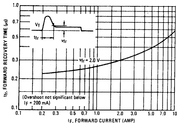
FIGURE 13 – FORWARD RECOVERY TIME
