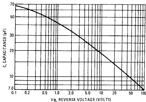
FIGURE 16 – JUNCTION CAPACITANCE
