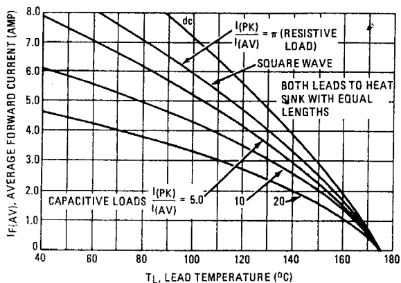
FIGURE 5 – 1/8" LEAD LENGTH
