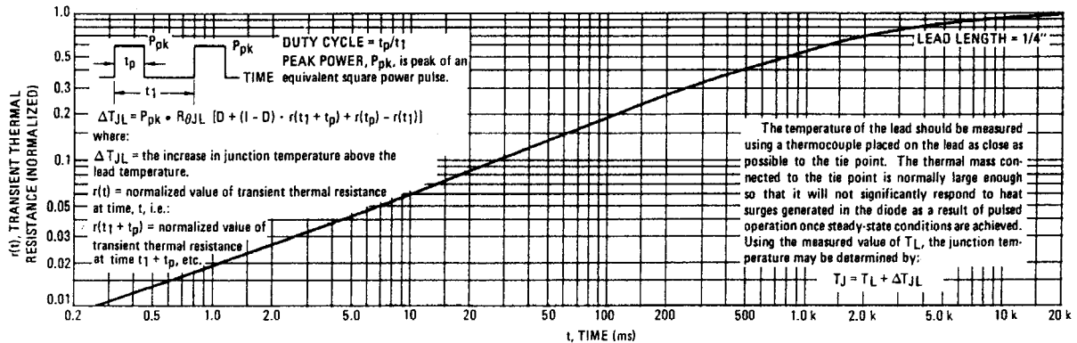
FIGURE 10 — THERMAL RESPONSE
