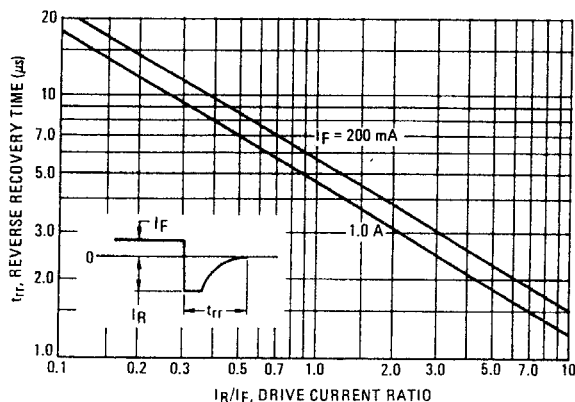
FIGURE 14 – REVERSE RECOVERY TIME
