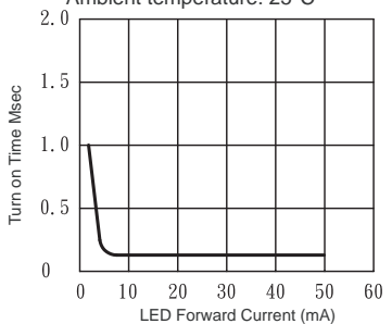
Fig.10 LED forward current vs. turn on time Across terminals 4 and 6 pin; Load voltage: 200V (DC); Continuous load current: 180mA (DC); Ambient temperature: 25°C
