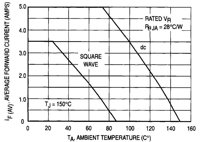
Figure 8. Current Derating Ambient (Mounting method #3 per note 1)
