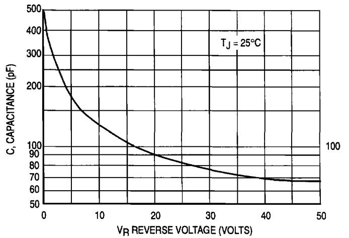
Figure 5. Typical Capacitance
