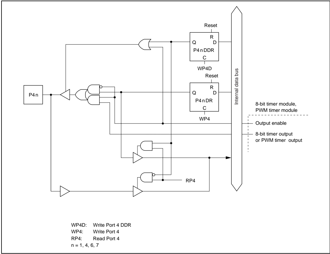
Figure 6.4 (b) Port 4 Schematic Diagram (Pins P4 1 , P4 4 , P4 6 , and P4 7 )
