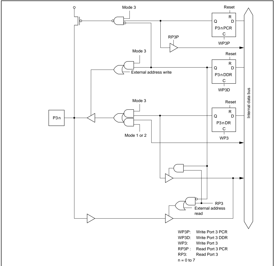
Figure 6.3 Port 3 Schematic Diagram
