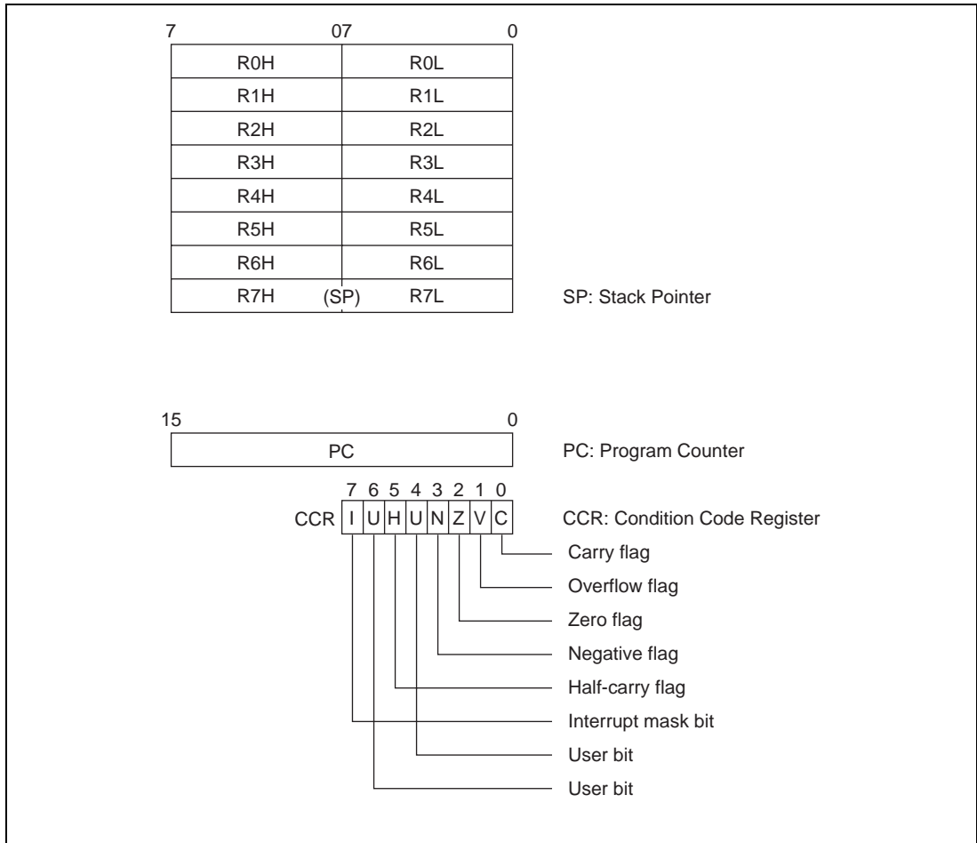
Figure 2.1 CPU Registers
