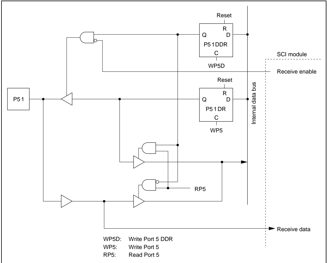
Figure 6.5 (b) Port 5 Schematic Diagram (Pin P5 1 )
