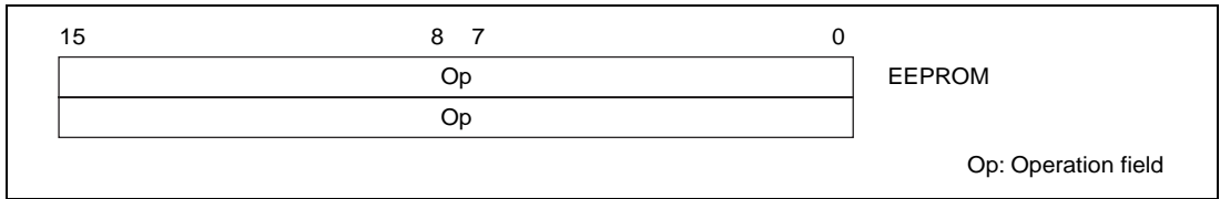
Figure 2.10 Block Data Transfer Instruction/EEPROM Write Operation Code
