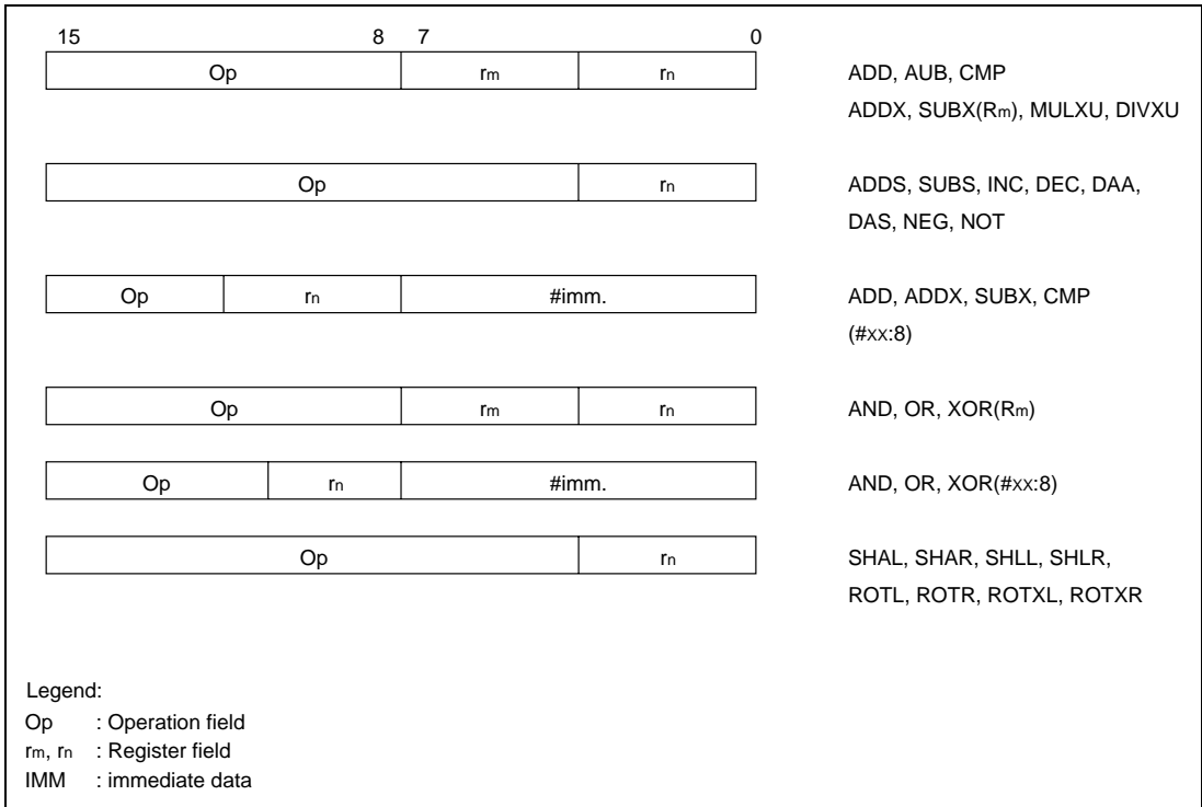
Figure 2.6 Arithmetic, Logic, and Shift Instruction Codes
