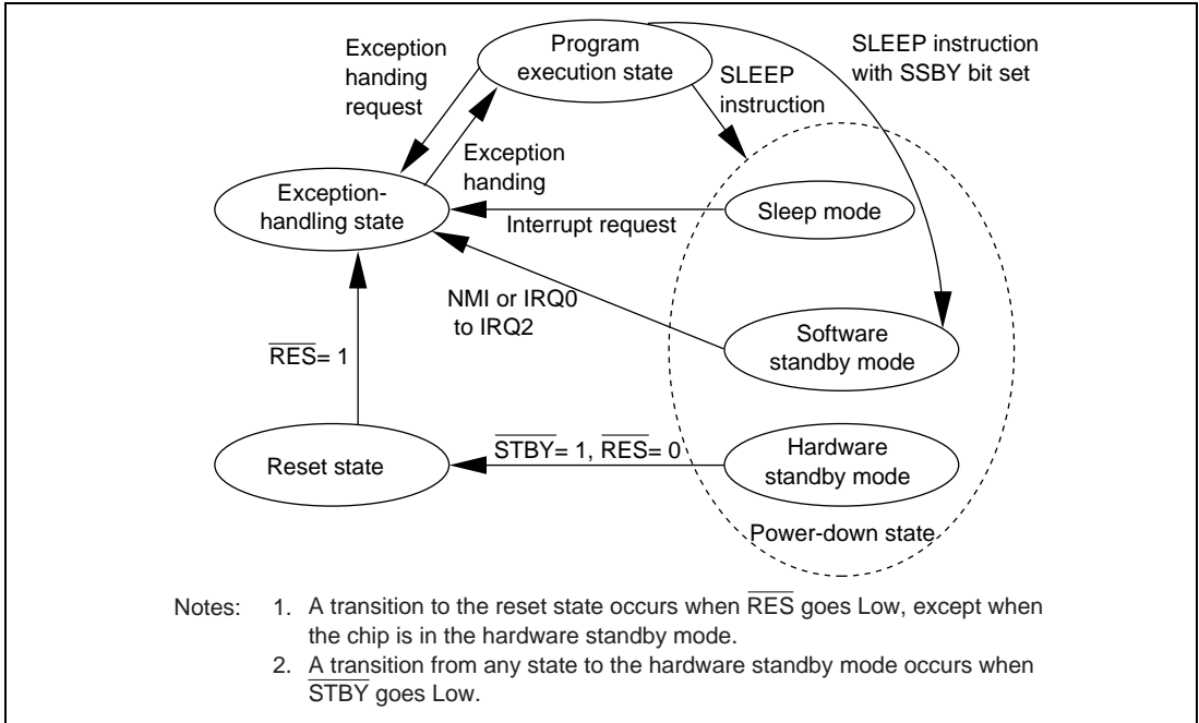
Figure 2.12 State Transitions
