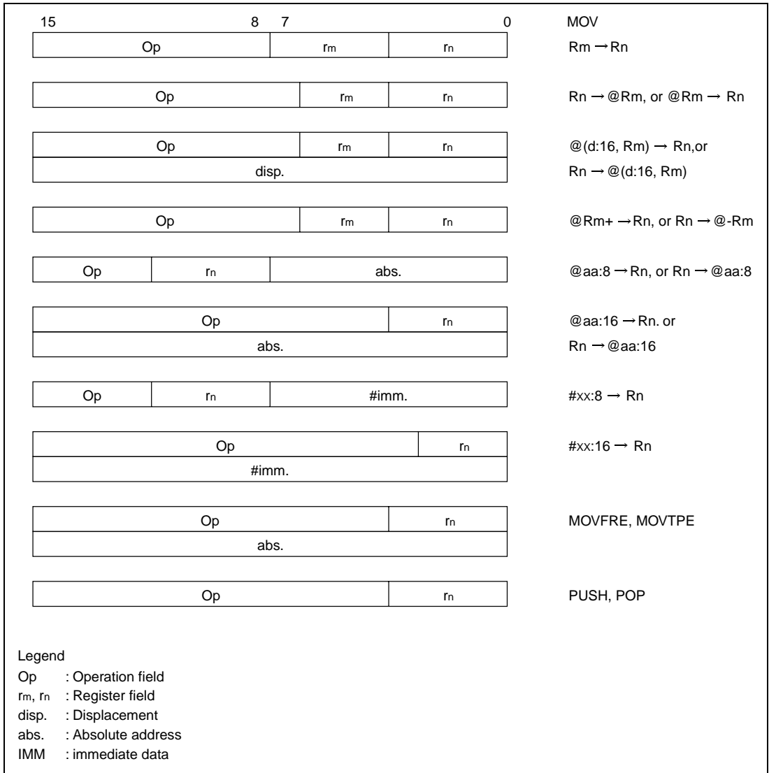
Figure 2.5 Data Transfer Instruction Codes
