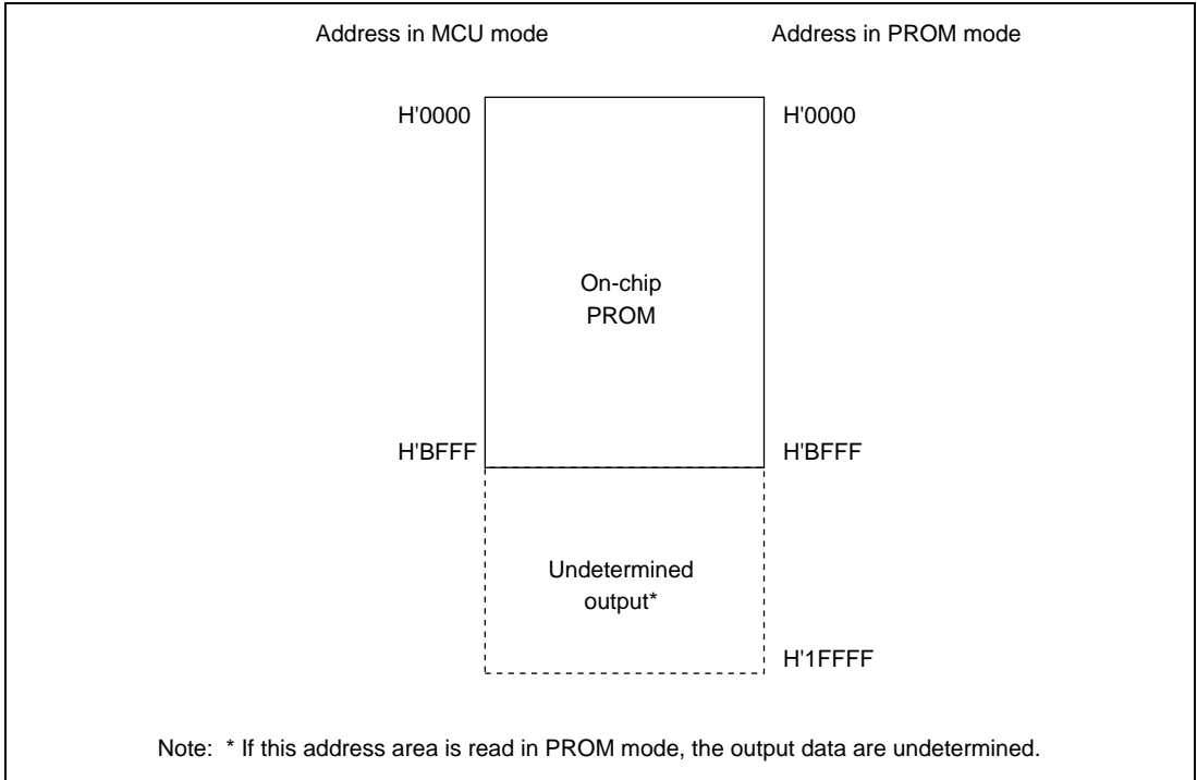
Figure 14.3 H8/338 Memory Map in PROM Mode
