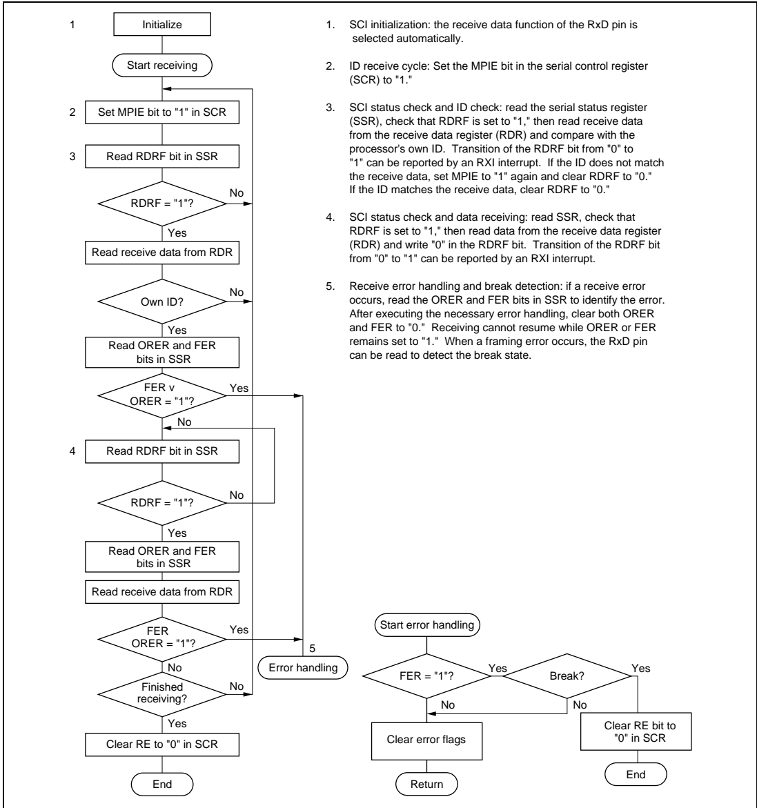
Figure 10.10 Sample Flowchart for Receiving Multiprocessor Serial Data
