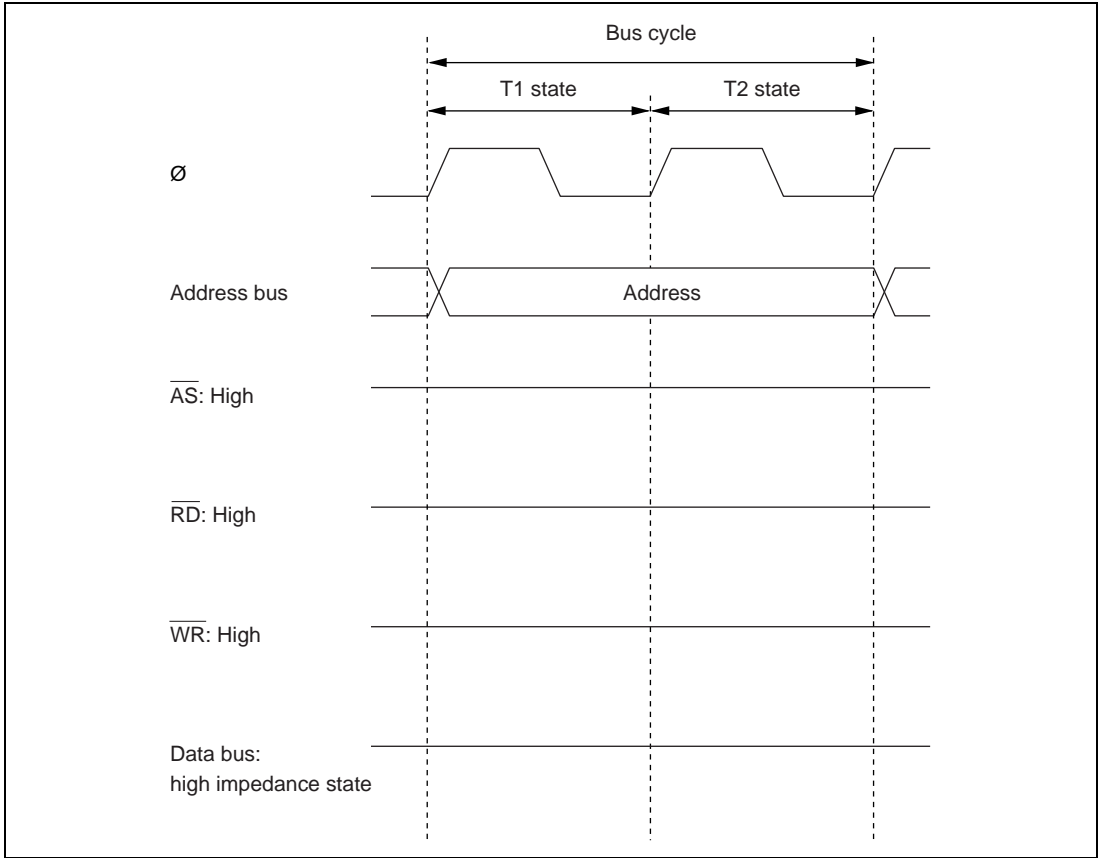
Figure 2.14 Pin States during On-Chip Memory Access Cycle
