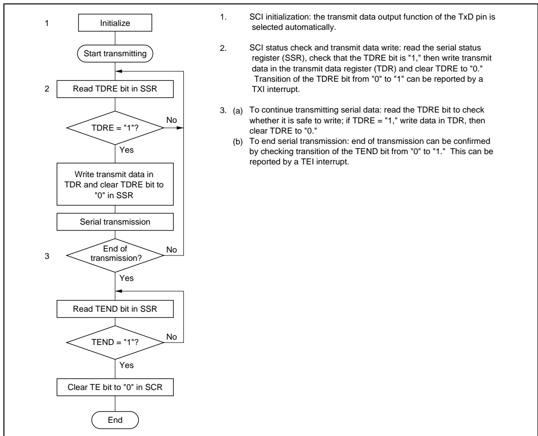
Figure 10.13 Sample Flowchart for Serial Transmitting
