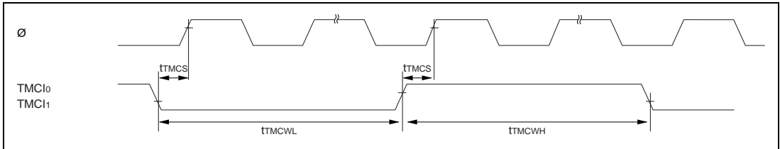
Figure 16.13 8-Bit Timer Clock Input Timing
