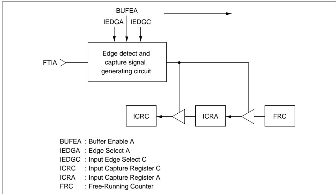
Figure 7.2 Input Capture Buffering
