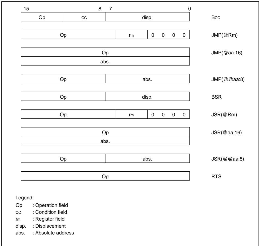
Figure 2.8 Branching Instruction Codes
