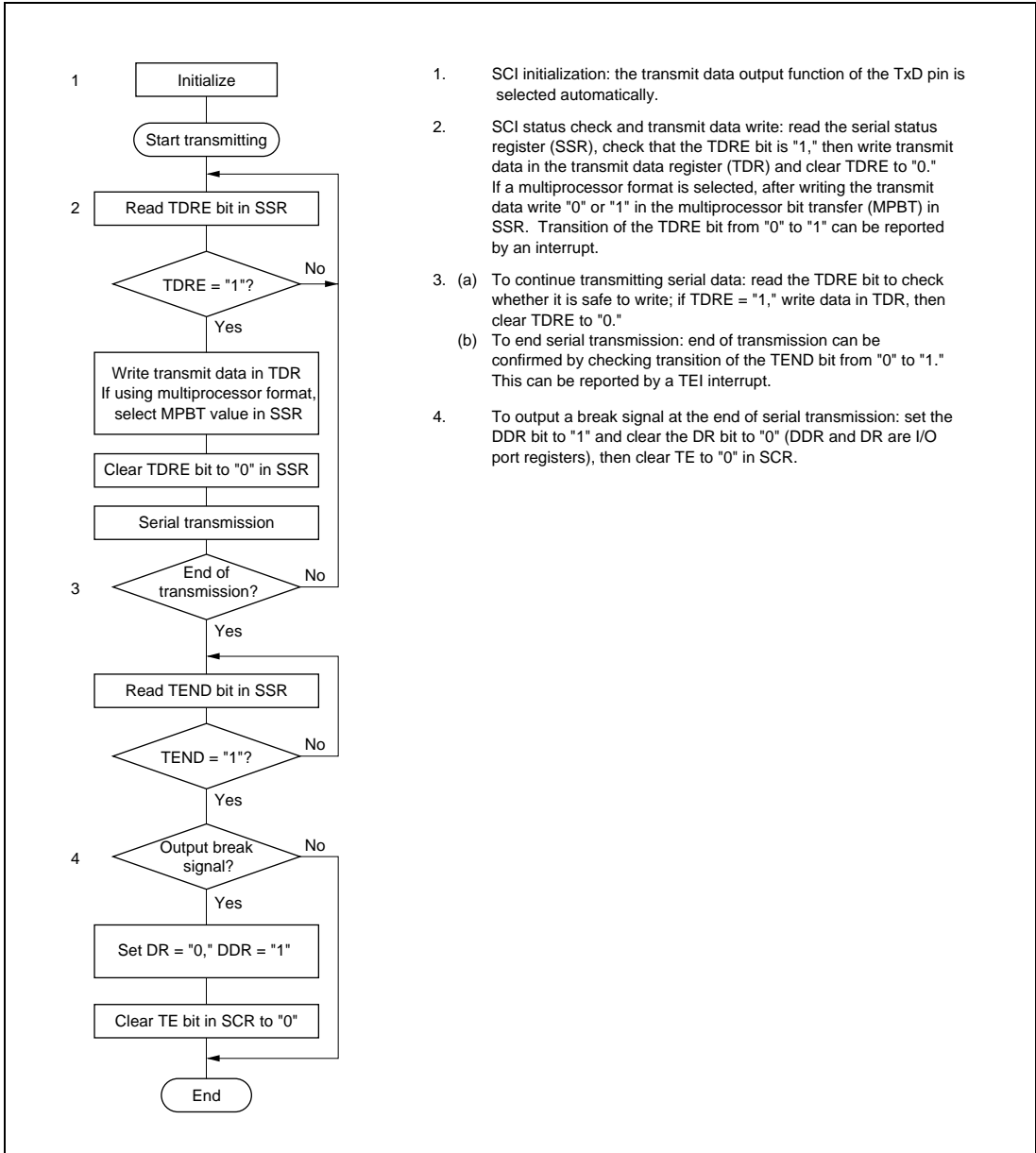
Figure 10.5 Sample Flowchart for Transmitting Serial Data
