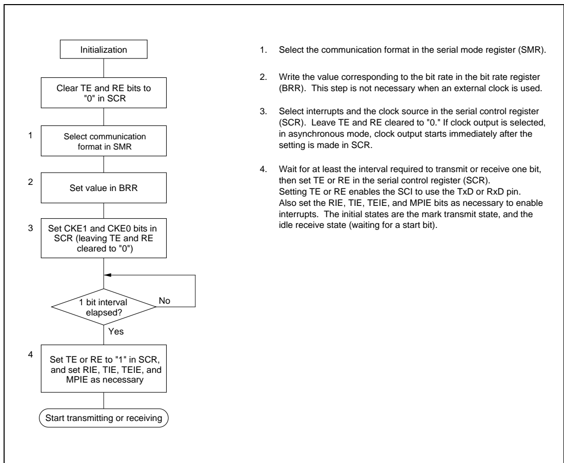
Figure 10.4 Sample Flowchart for SCI Initialization
