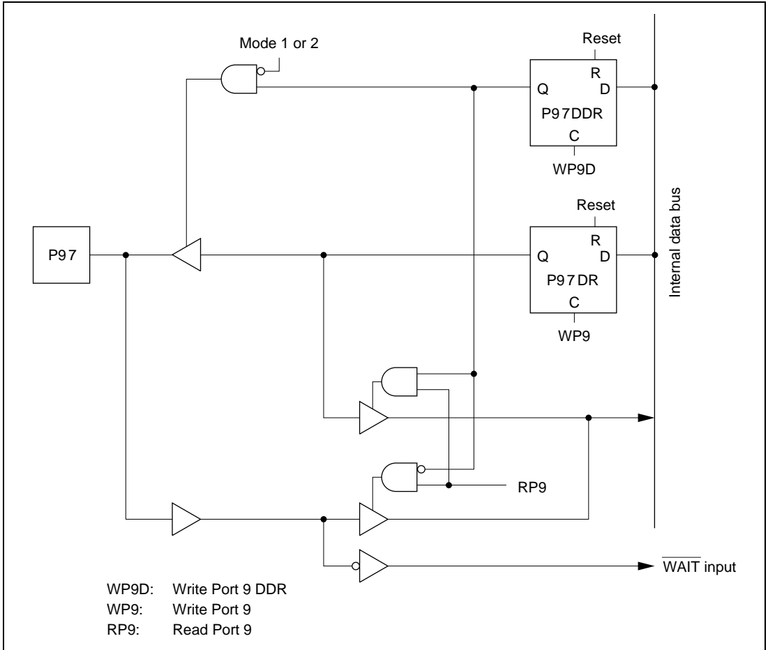
Figure 6.9 (e) Port 9 Schematic Diagram (Pin P97)
