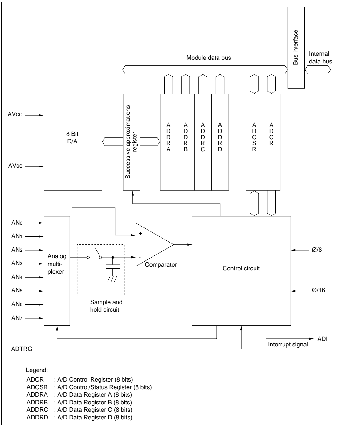
Figure 11.1 Block Diagram of A/D Converter
