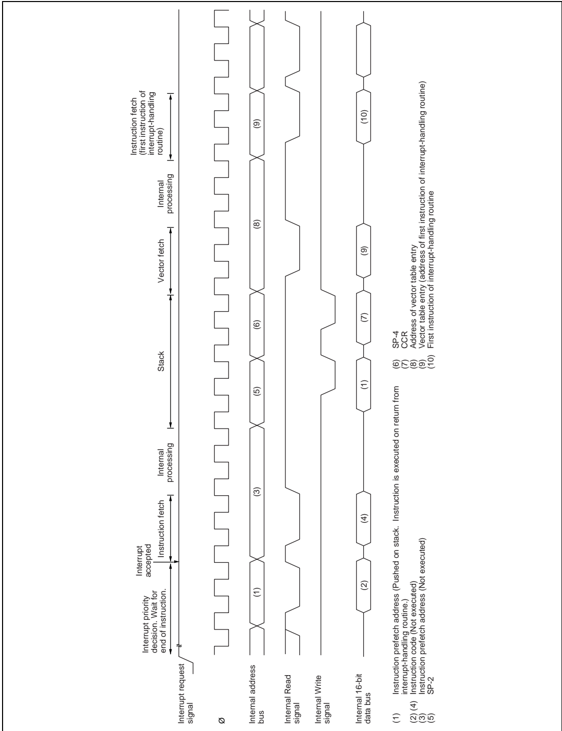
Figure 4.6 Timing of Interrupt Sequence
