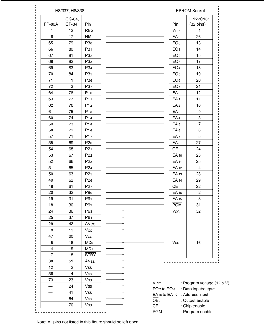
Figure 14.2 Socket Adapter Pin Assignments
