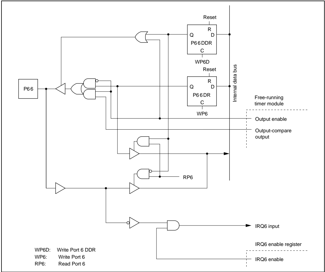
Figure 6.6 (c) Port 6 Schematic Diagram (Pin P6 6 )
