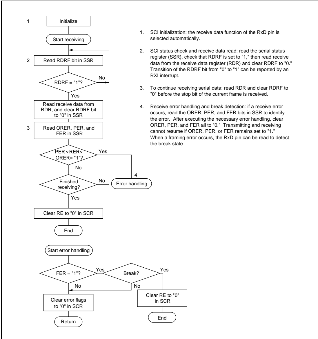
Figure 10.7 Sample Flowchart for Receiving Serial Data
