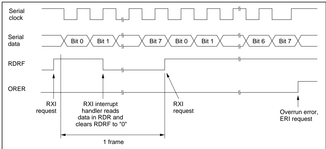
Figure 10.16 Example of SCI Receive Operation
