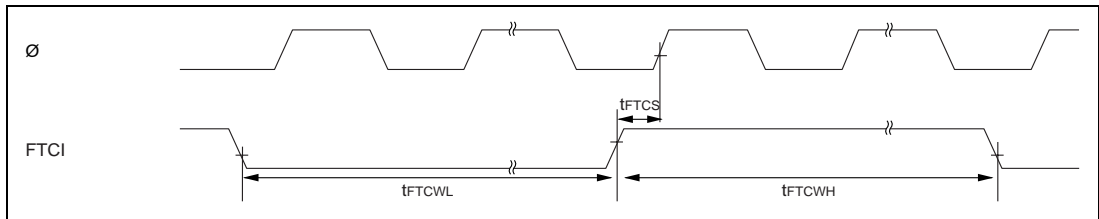
Figure 16.11 External Clock Input Timing for Free-Running Timer
