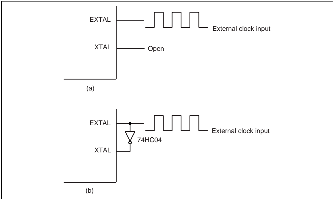
Figure 5.5 External Clock Input (Example)
