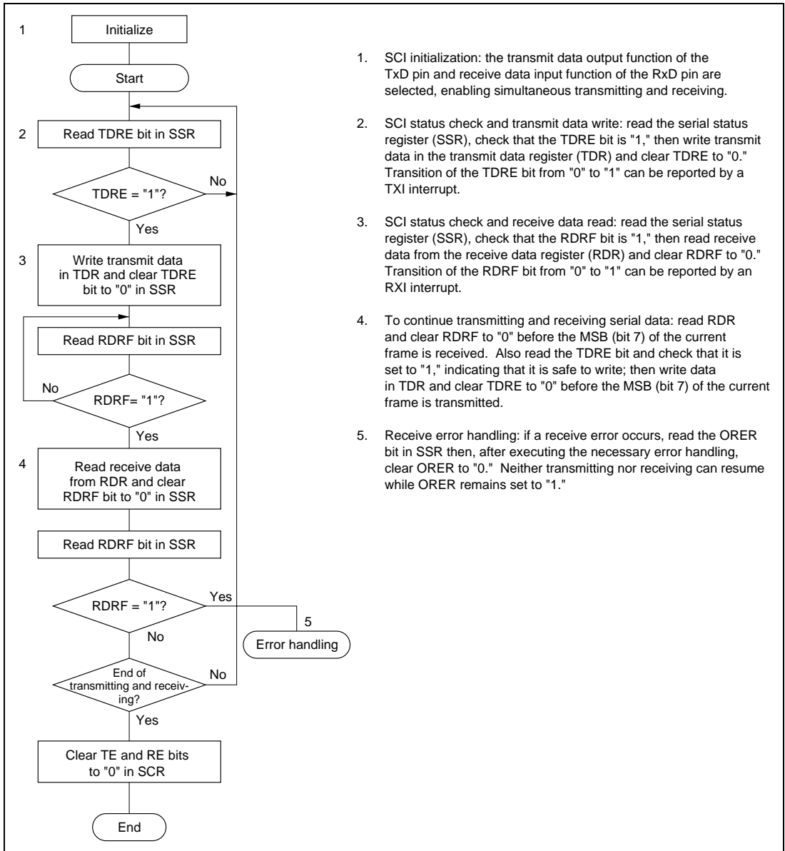
Figure 10.17 Sample Flowchart for Serial Transmitting and Receiving
