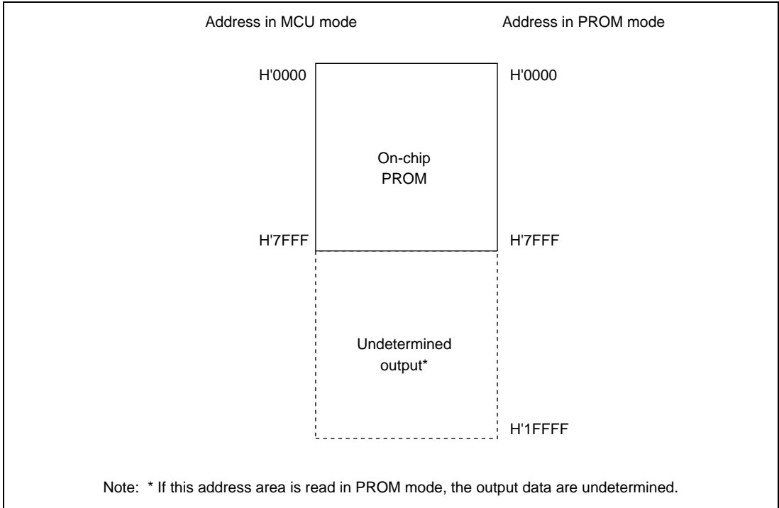
Figure 14.4 H8/337 Memory Map in PROM Mode
