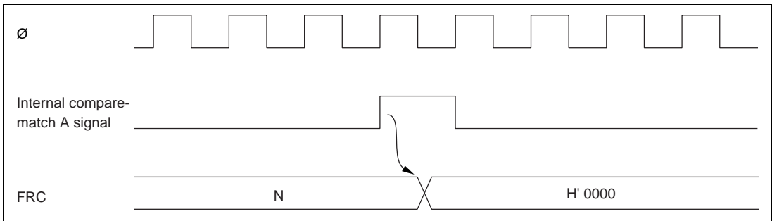
Figure 7.7 Setting of Output Compare Flags
