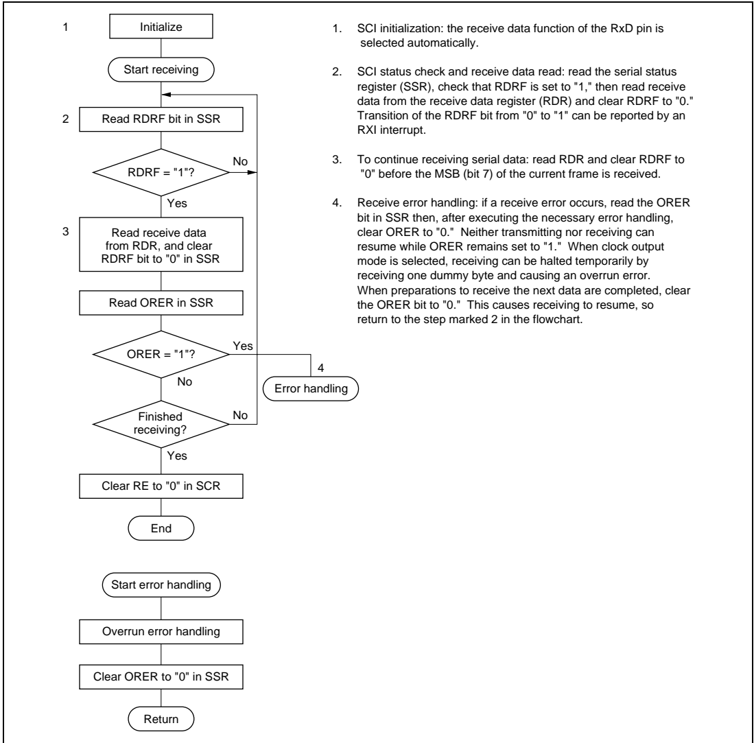
Figure 10.15 Sample Flowchart for Serial Receiving
