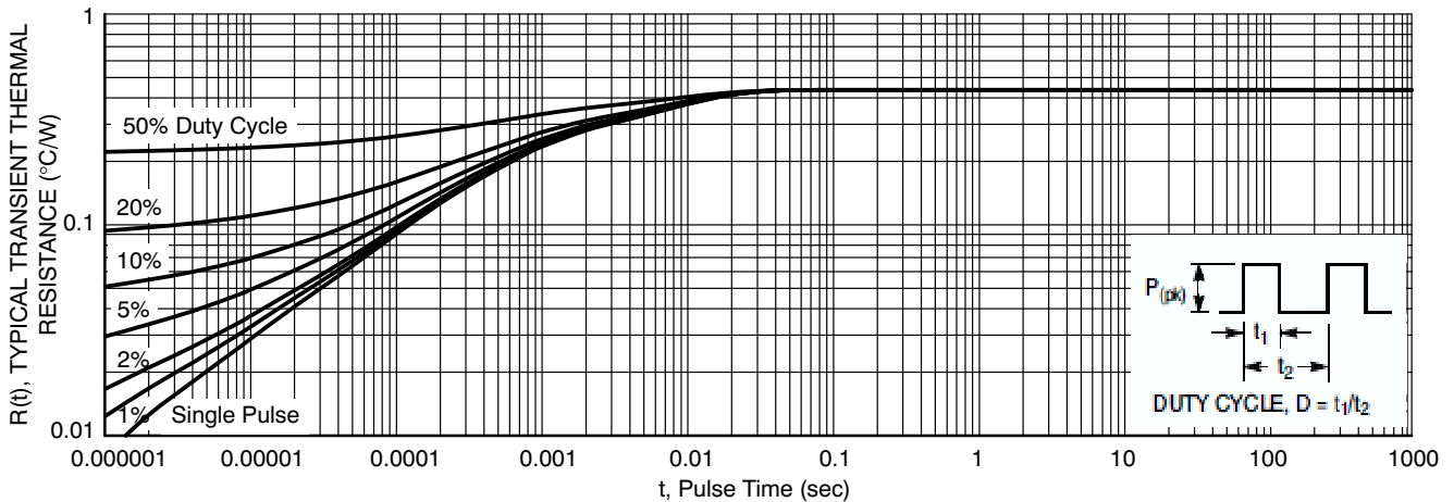
Figure 9. Typical Transient Thermal Response for NTSB20U100CTG
