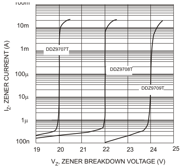
Fig. 7 Typical Reverse Characteristics, DDZ9707T - DDZ9709T
