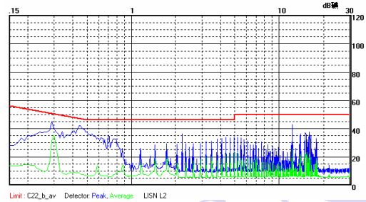
WRB2405MT-3W CE(Class B, Negative line)
