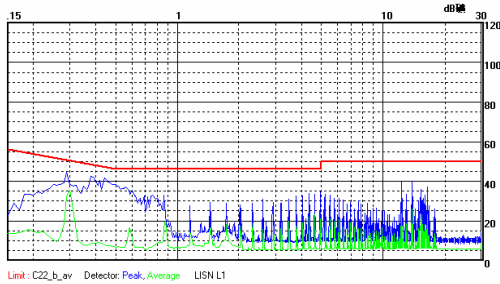
WRB2405MT-3W CE(Class B, Positive line)
