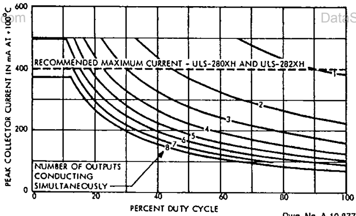
Dwg. No. A-10,877A
