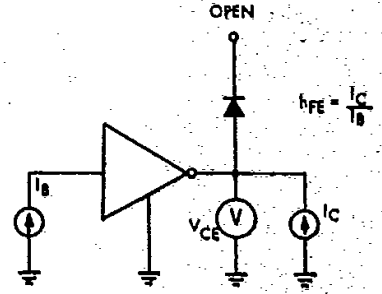
Dwg. No. A-9731
