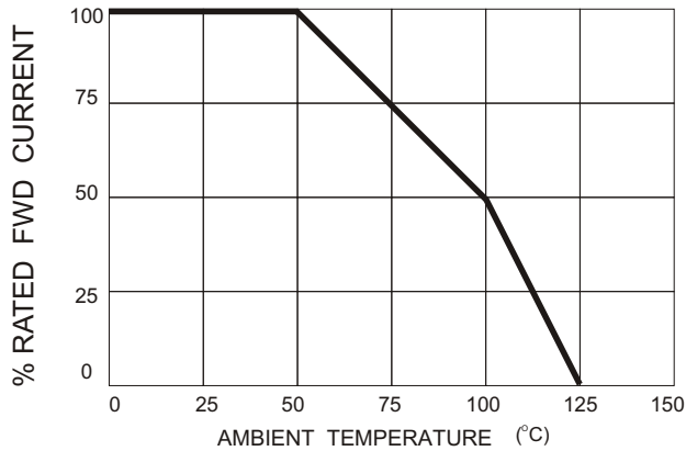
OUTPUT CURRENT vs AMBIENT TEMPERATURE
