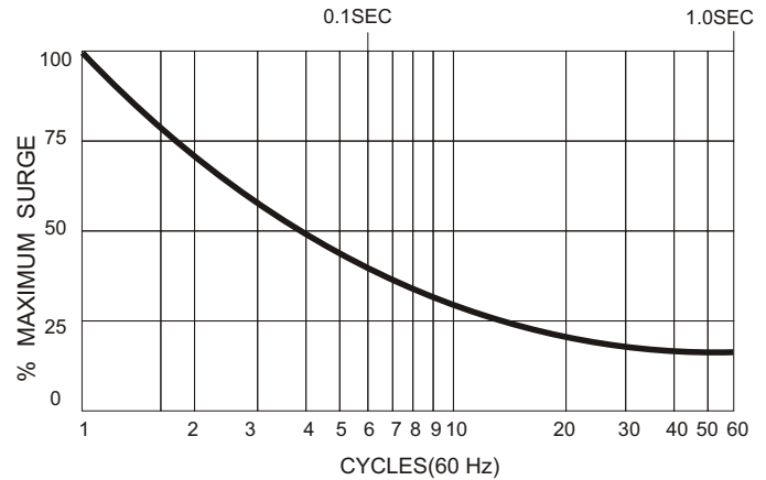
NON-REPETITIVE SURGE CURRENT RATINGS
