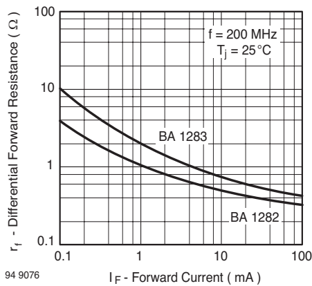
Fig. 1 Differential Forward Resistance vs. Forward Current
