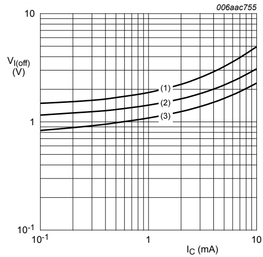
V_{CE} = 5 V (1) T_{amb} = -40^\circ C (2) T_{amb} = 25^\circ C (3) T_{amb} = 100^\circ C
