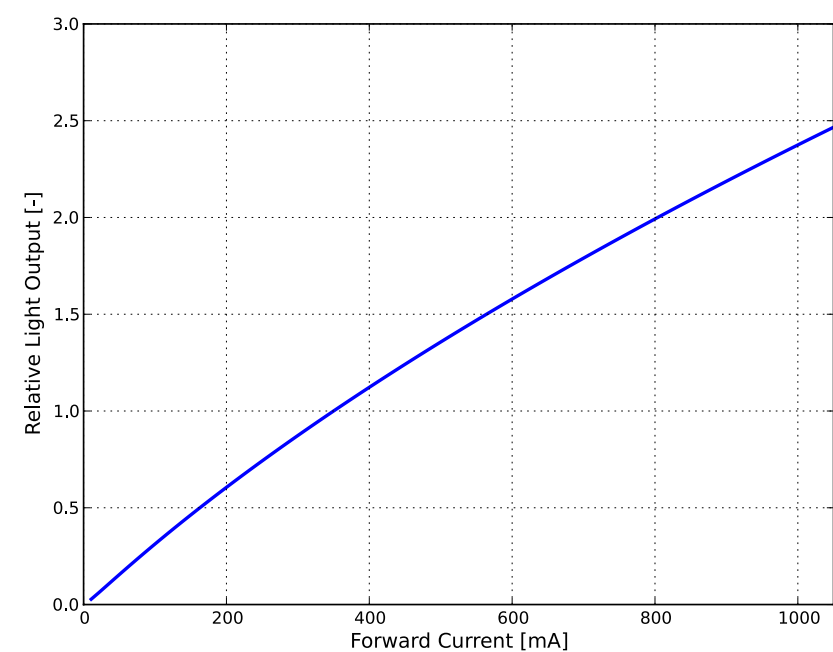
Figure 7. Typical relative luminous flux vs. forward current, LIQ0-xyy00000zzz0.
