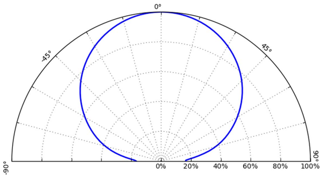
Figure 10. Typical representative polar radiation pattern for LIQ0-xyyy00000zzz0.
