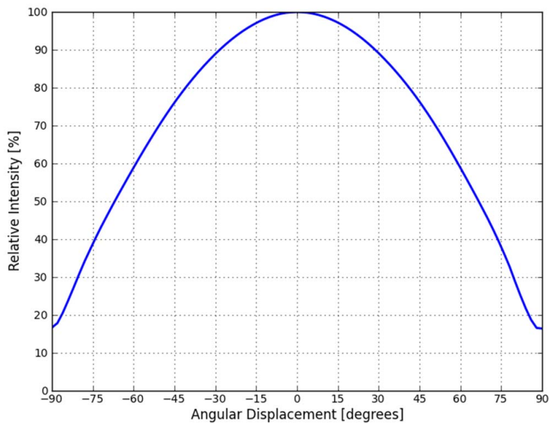
Figure 9. Typical representative spatial radiation pattern for LIQ0-xyyy00000zzz0.
