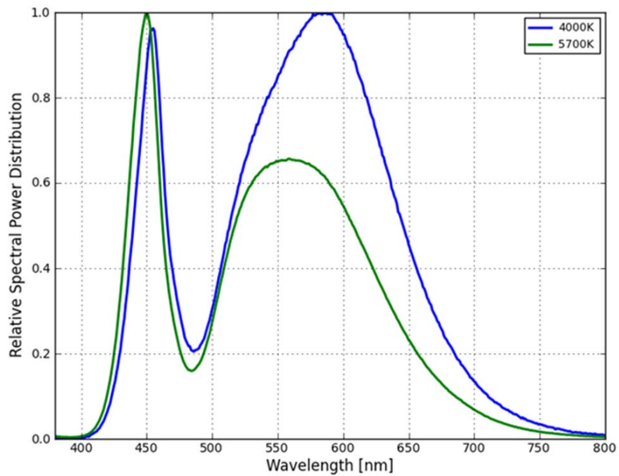
Figure 5. Color Spectrum of LIQ0-xx7000000zzz0.
