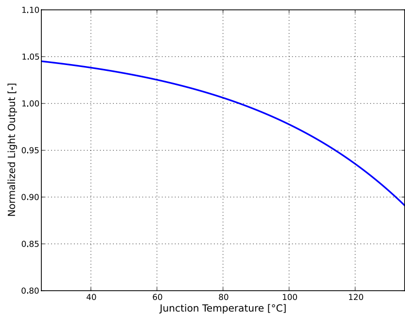
Figure 6. Relative light output vs. junction temperature, LIQ0-xyy00000zzz0.
