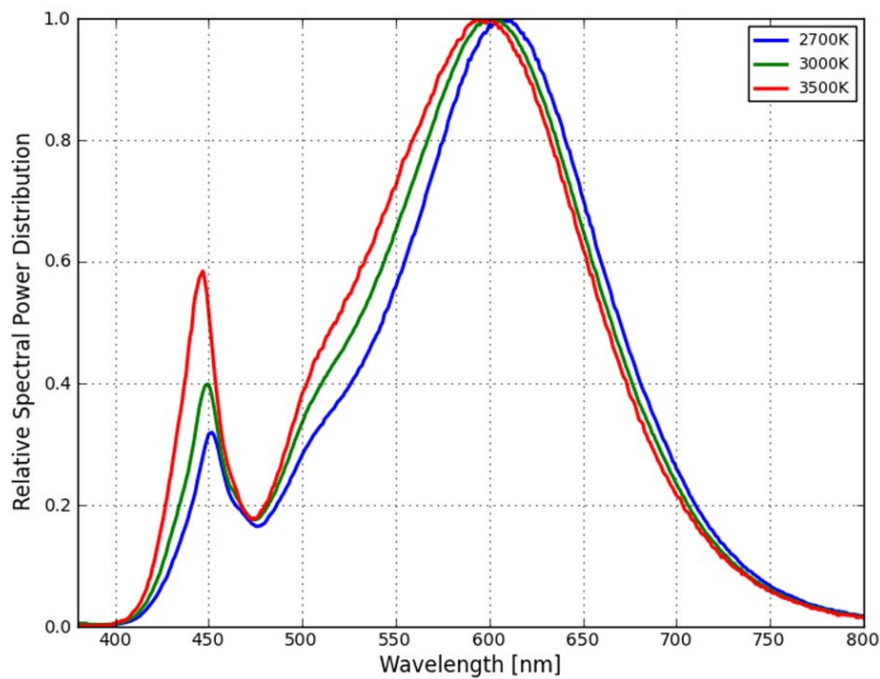
Figure 4. Color Spectrum of LIQ0-xx8000000zzz0.
