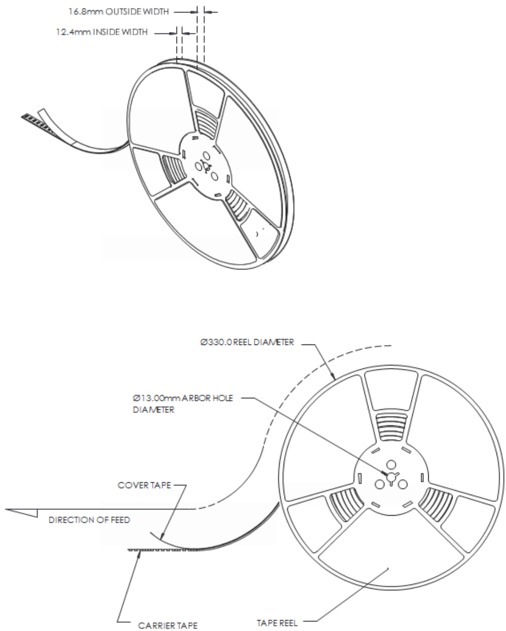
Figure 12. Emitter reel packaging.
