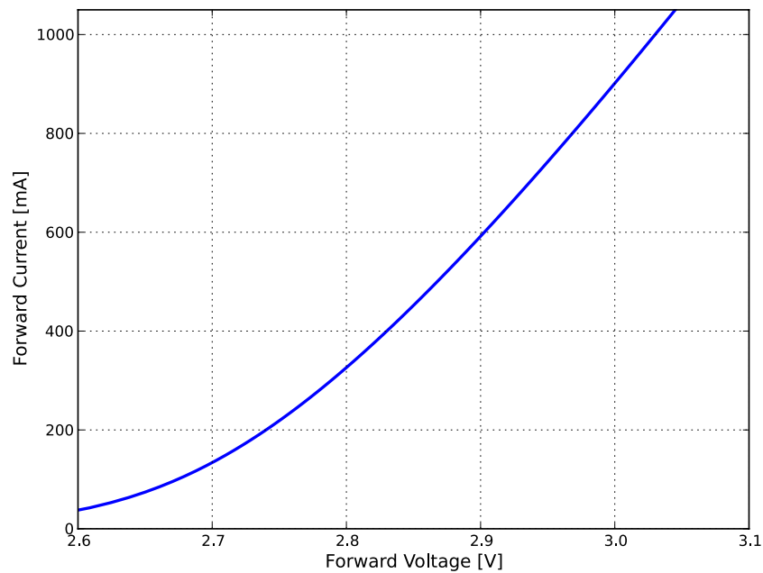
Figure 8. Typical forward current vs. forward volatage, L I Q0-xyy00000zzz0.
