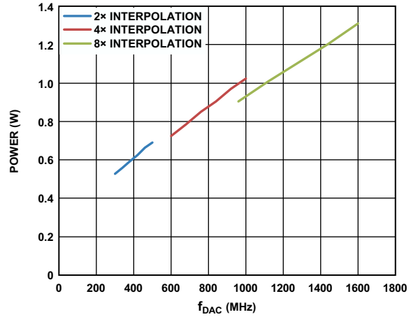
Figure 24. Total Power Consumption vs. f_{DAC} over Interpolation
