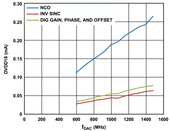
Figure 26. DVDD18 Current vs. f_{DAC} over Digital Functions
