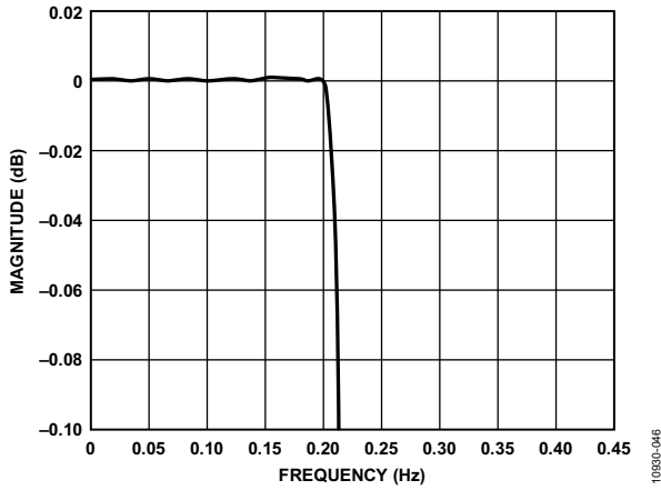
Figure 41. Pass-Band Detail of 4× Mode
