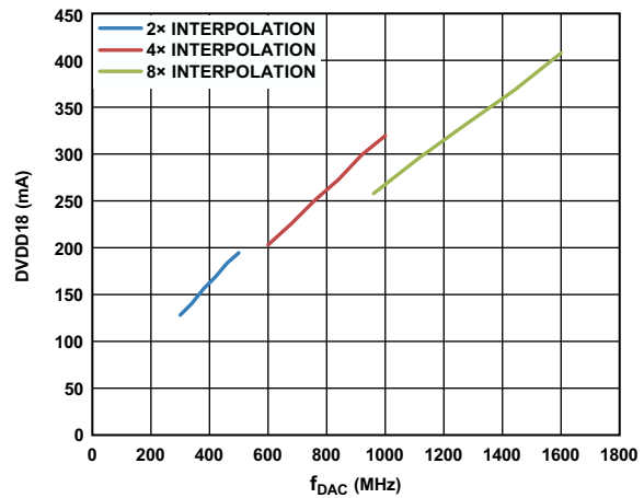
Figure 25. DVDD18 Current vs. f_{DAC} over Interpolation
