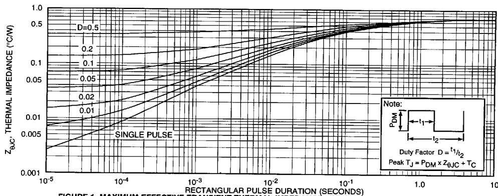
FIGURE 1. MAXIMUM EFFECTIVE TRANSIENT THERMAL IMPEDANCE, JUNCTION-TO-CASE vs PULSE DURATION Page 159
