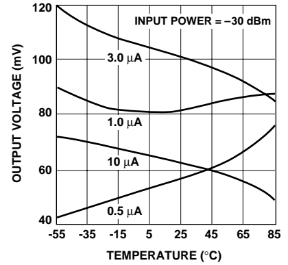
Figure 20. Output Voltage vs. Temperature and Bias Current in the 915 MHz Voltage Doubler using the HSMS-286a Series.
