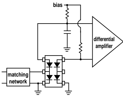
Figure 19. Differential Voltage Doubler, HSMS-286P.
