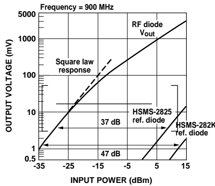
Figure 18. Comparing HSMS-282K with HSMS-2825.
