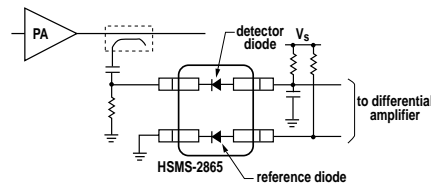
Figure 14. Conventional Differential Detector.
