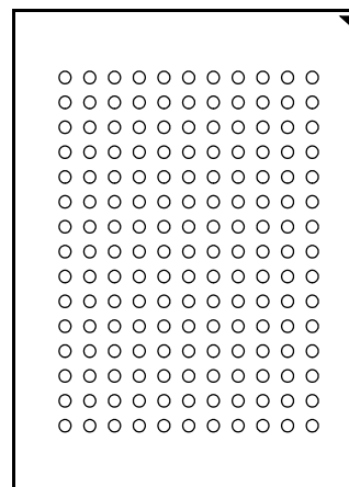
Bottom View 165-Bump, 13 mm x 15 mm BGA 1 mm Bump Pitch, 11 x 15 Bump Array
