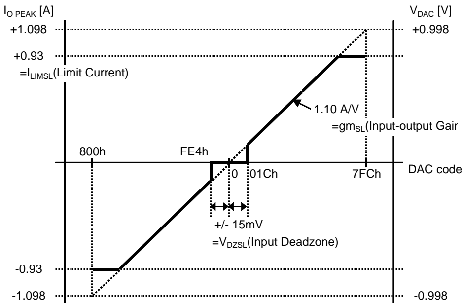
Figure 12. I_{O\ PEAK} Characteristics (When set as R_{SLRNF}=0.56 \Omega ).
