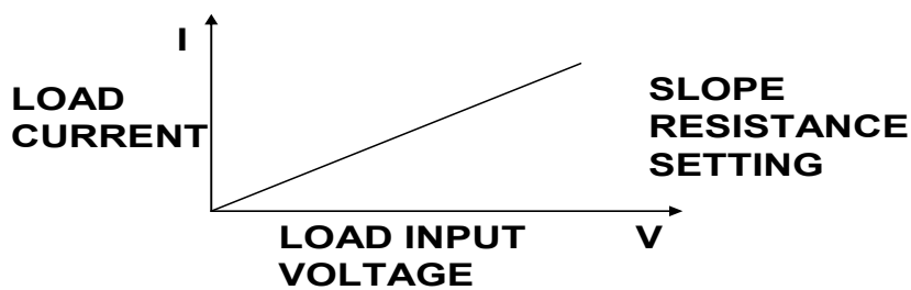
CONSTANT RESISTANCE MODE
