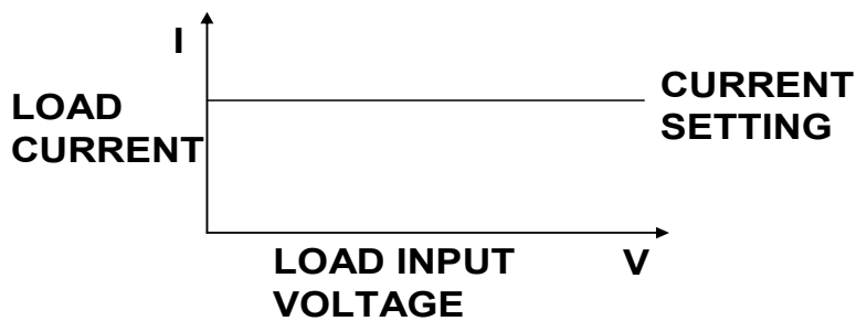
CONSTANT CURRENT MODE
