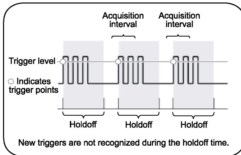
Figure 5.3: Trigger holdoff
