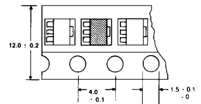
SOT-223 TAPE DIMENSIONS AND ORIENTATION
