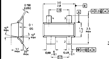
SOT-143 TOP VIEW
