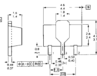
SOT-89 BOTTOM VIEW
