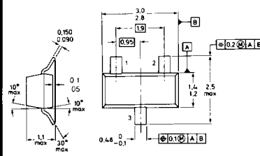
SOT-23 TOP VIEW
