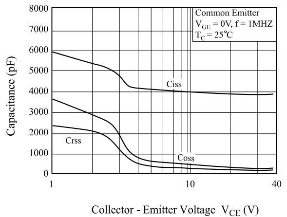
Fig 6. Capacitance Characteristics
