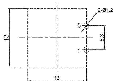
P.C.B.LAYOUT(BottomView)
