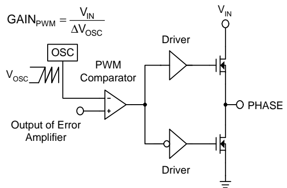
Figure 5. The PWM Modulator
