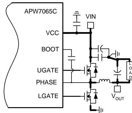
Figure 8. Layout Guidelines
