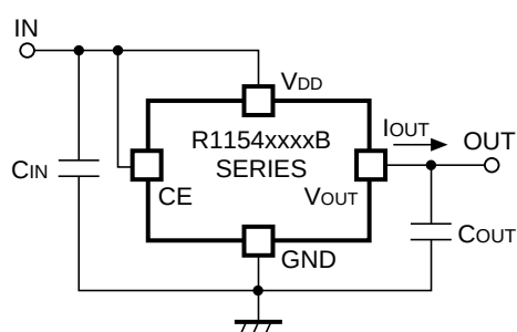
R1154xxxB Standard Test Circuit
