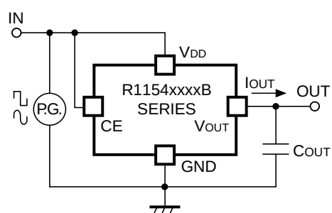
R1154xxxB Input Transient Response Test Circuit
