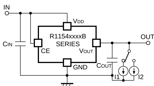
R1154xxxB Load Regulation Test Circuit
