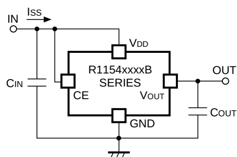
R1154xxxB Supply Current Test Circuit
