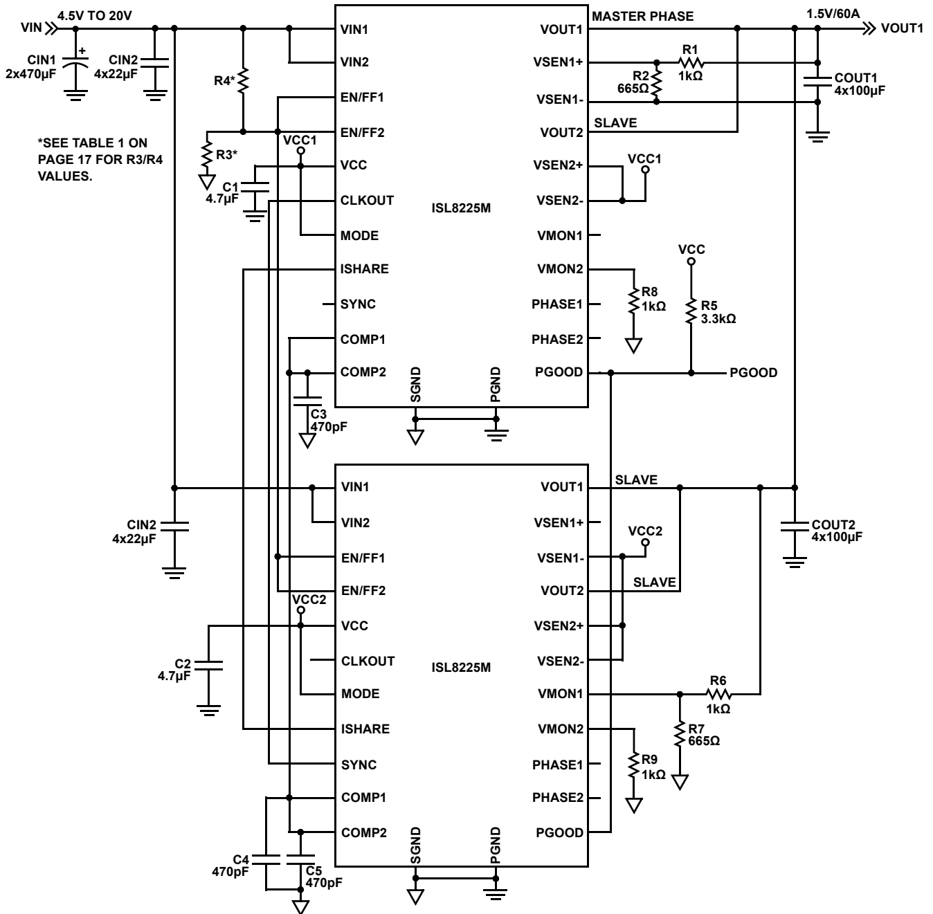
FIGURE 22. 4-PHASE PARALLELED AT 1.5V/60A WITH 90° INTERLEAVING
