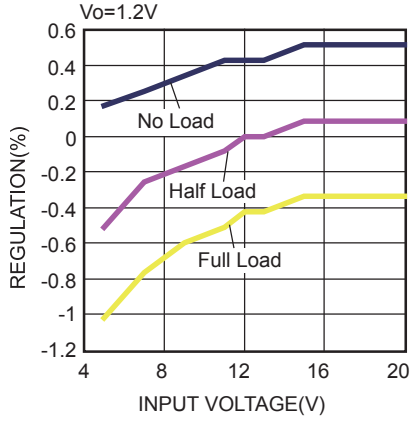
Line Regulation
