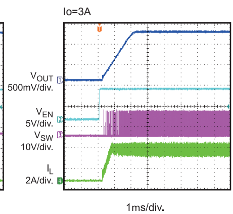
Start Up Through EN
