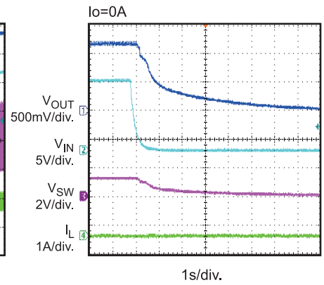
Shut Down Through Vin
