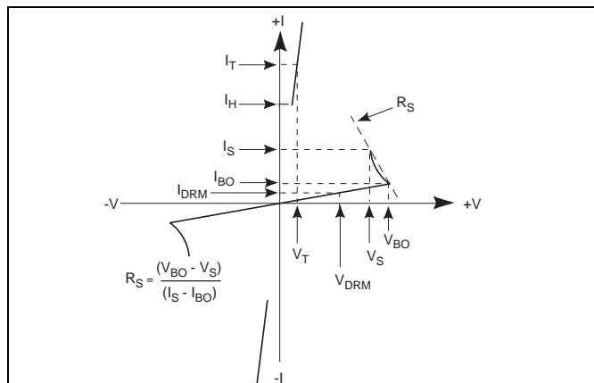
V-I Characteristics
