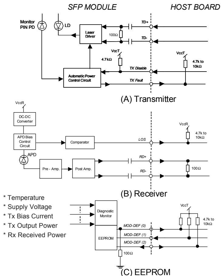
Figure 1. Block Diagram (Diagnostic Monitor is incorporated for SCP6EC4-GL-#N-xx only.)
