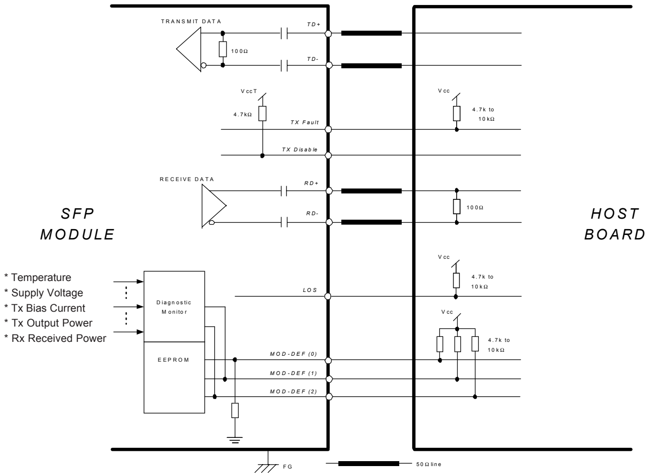
Figure 13. Recommended Interface Circuit (Diagnostic Monitor is incorporated for SCP6EC4-GL-#N-xx only.)
