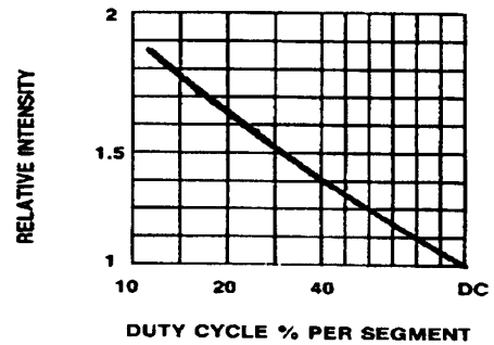
Fig.5 LUMINOUS INTENSITY VS. DUTY CYCLE
