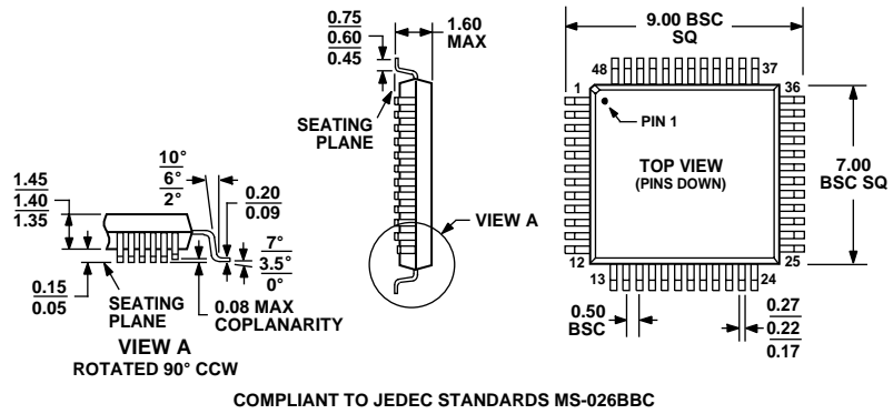
Figure 58. 48-Lead Low Profile Quad Flat Package [LQFP] (ST-48) Dimensions shown in inches millimeters
