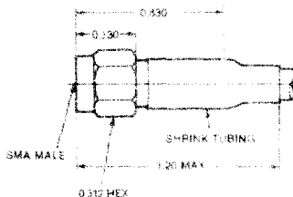
Straight Cable Male (crimp or solder attachment)
