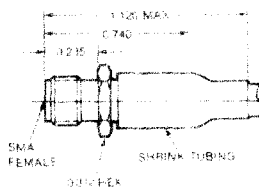
Straight Cable Female (crimp or solder attachment)
