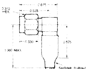
Right Angle Cable Male (crimp or solder attachment)
