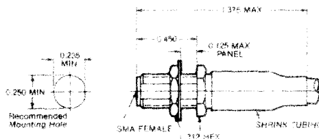
Bulkhead Feedthrough Cable Female (crimp or solder attachment)
