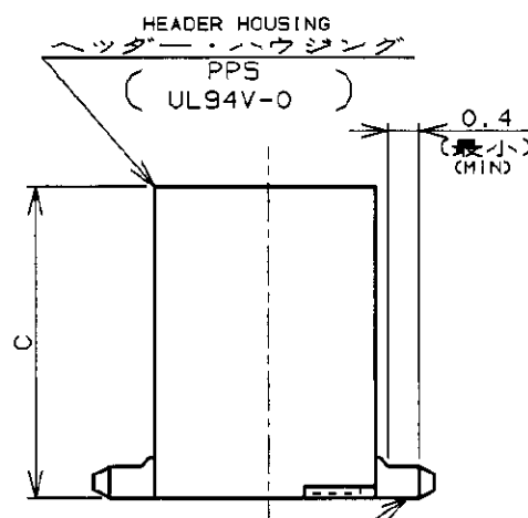
POST ポスト (半田めっき仕上げ黄銅線) POST-TIN-LEAD BRASS WIRE 0.5 DIA
