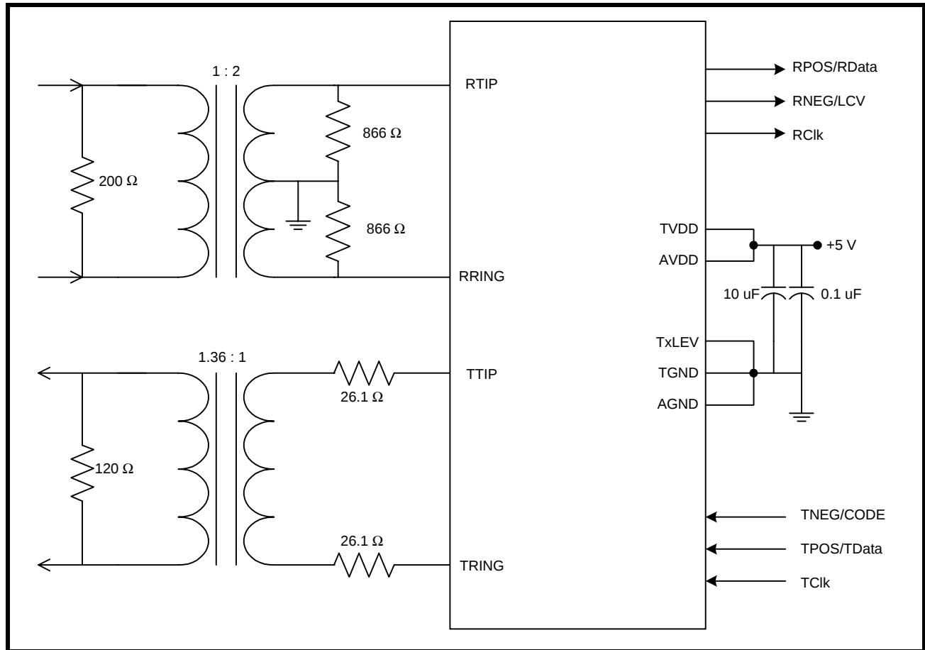
FIGURE 13. RECOMMENDED SCHEMATIC FOR TRANSFORMER-COUPPLING THE XRT82D20 TO THE LINE FOR 120 \Omega APPLICATIONS AND 5 V OPERATION ONLY
