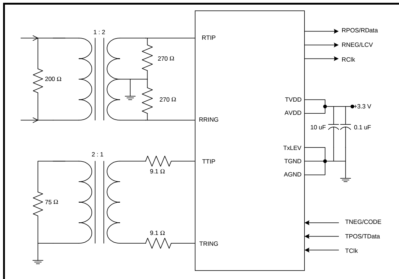
FIGURE 10. ILLUSTRATION OF HOW TO INTERFACE THE XRT82D20 TO THE LINE FOR 75 \Omega APPLICATIONS AND 3.3V OPERATION ONLY
