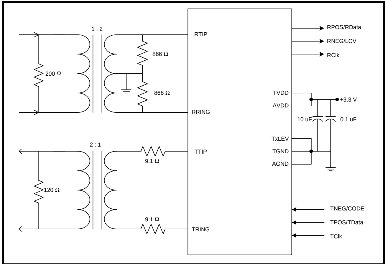
FIGURE 11. ILLUSTRATION OF HOW TO INTERFACE THE XRT82D20 TO THE LINE FOR 120 \Omega APPLICATIONS AND 3.3V OPERATION ONLY
