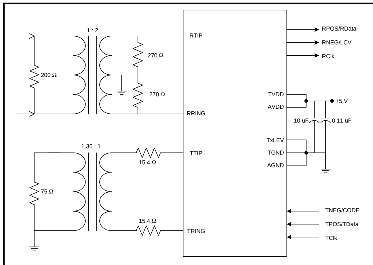
FIGURE 12. RECOMMENDED SCHEMATIC FOR TRANSFORMER-COUPPLING THE XRT82D20 TO THE LINE FOR 75 \Omega APPLICATIONS AND 5 V OPERATION ONLY
