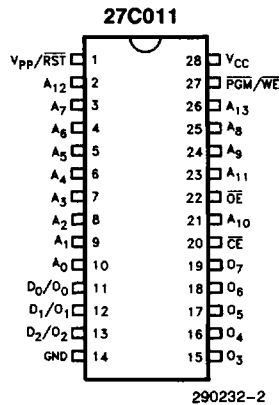
Figure 2. Pin Configuration
