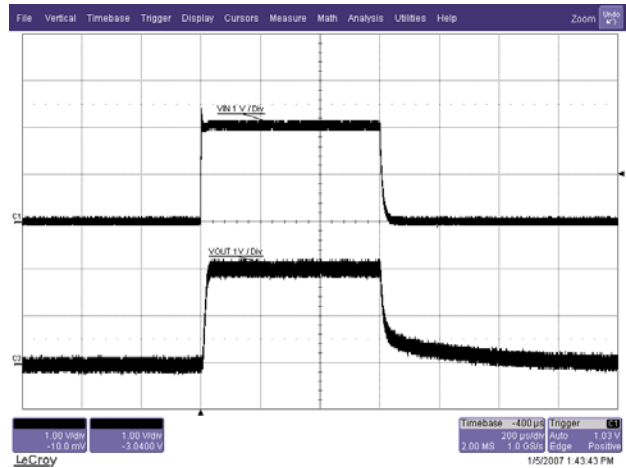
Figure 11. Turn-on Response
