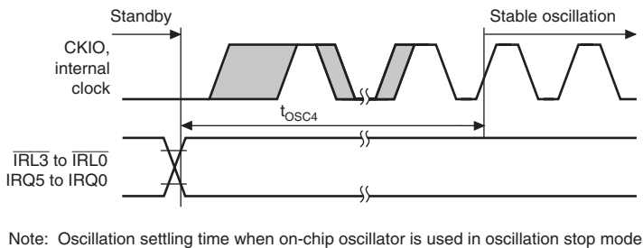
Figure 24.8 Oscillation Settling Time at Standby Return (Return by IRQ5 to IRQ0 and \overline{\text{IRL3}} to \overline{\text{IRL0}} )
