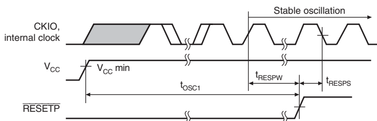
Figure 24.5 Power-On Oscillation Settling Time
