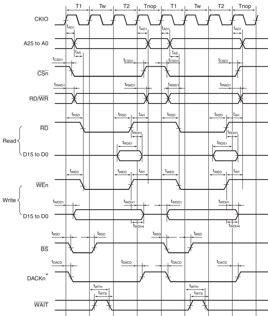
Figure 24.20 Basic Bus Cycle (One Software Wait, External Wait Enabled (WM bit = 0), No Idle Cycle Setting)
