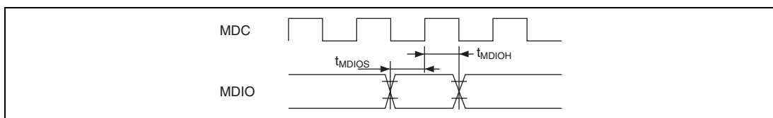
Figure 24.63 MDIO Input Timing
