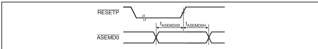
Figure 24.73 \overline{\text{ASEMD0}} Input Timing
