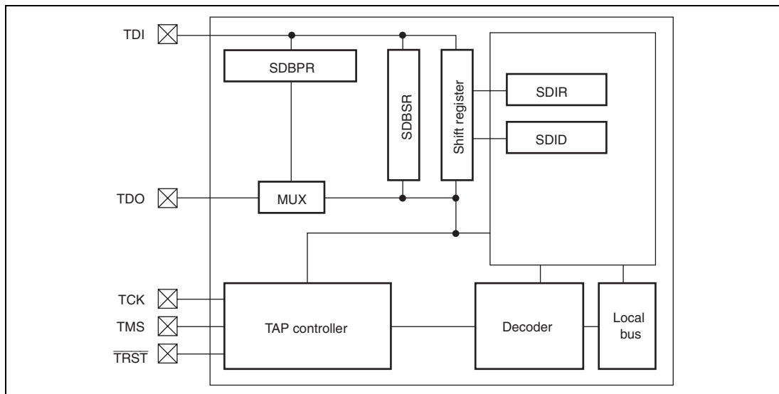
Figure 22.1 Block Diagram of H-UDI
