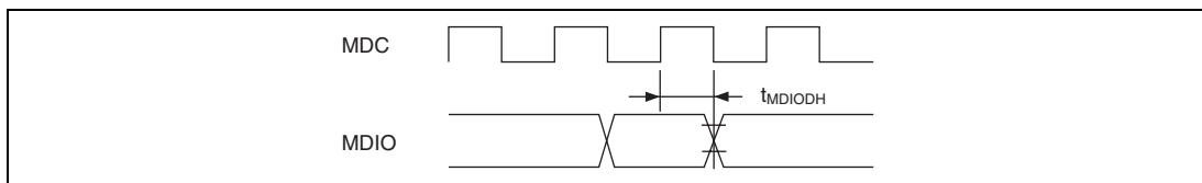
Figure 24.64 MDIO Output Timing
