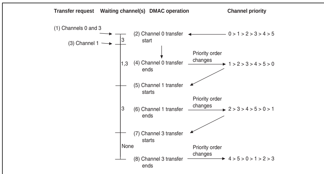
Figure 13.4 Changes in Channel Priority in Round-Robin Mode
