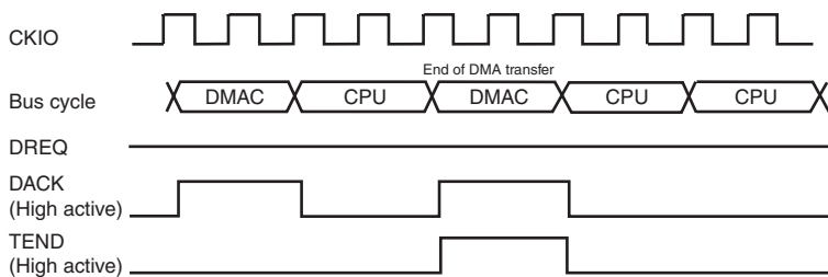
Figure 13.16 Example of DMA Transfer End Timing (Cycle Steal Level Detection)
