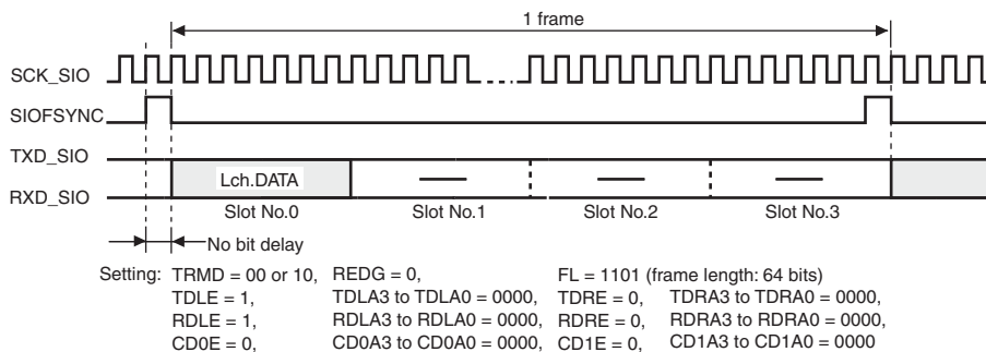
Figure 17.15 Transmission and Reception Timings (16-Bit Monaural Data (1))
