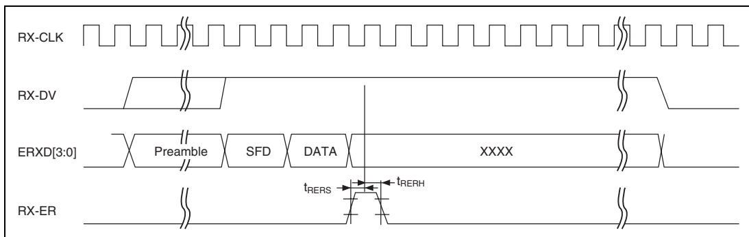
Figure 24.62 MII Receive Timing (Case of Error)
