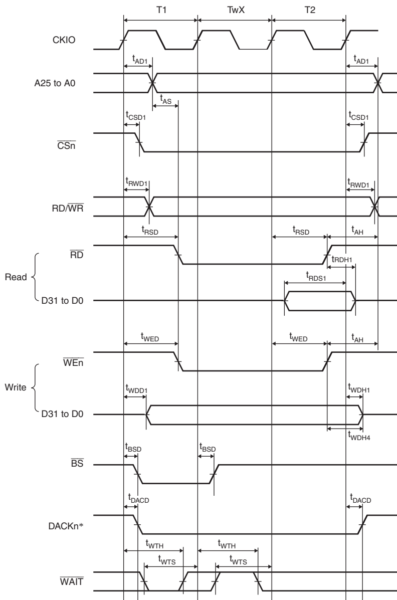
Figure 24.19 Basic Bus Cycle (One External Wait)
