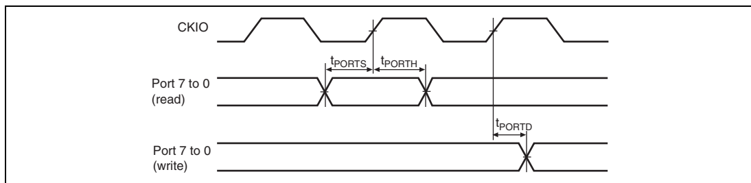
Figure 24.69 I/O Port Timing
