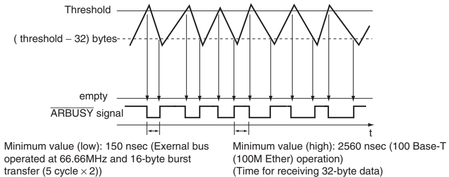
Figure 19.10 \overline{\text{ARBUSY}} Signal Change and Minimum Pulse Width Depending on Increase and Decrease of FIFO
