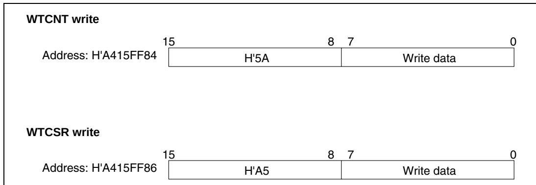
Figure 11.3 Writing to WTCNT and WTCSR
