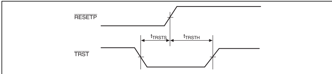
Figure 24.71 \overline{\text{TRST}} Input Timing (Reset Hold)
