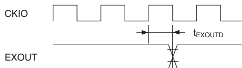
Figure 24.66 EXOUT Output Timing
