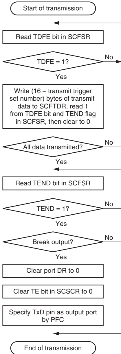
Figure 16.4 Sample Serial Transmission Flowchart
