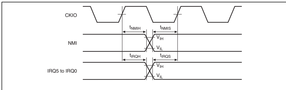
Figure 24.13 Interrupt Signal Input Timing
