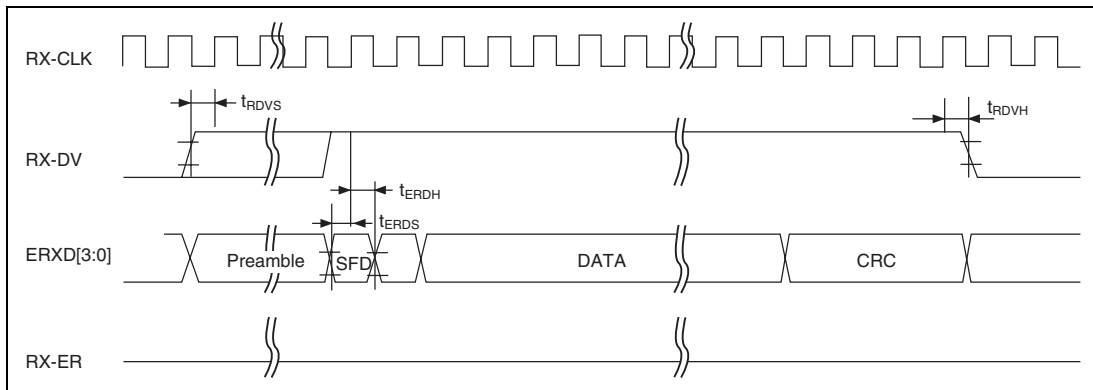
Figure 24.61 MII Receive Timing (Normal Operation)
