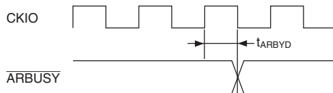
Figure 24.68 ARBUSY Output Timing
