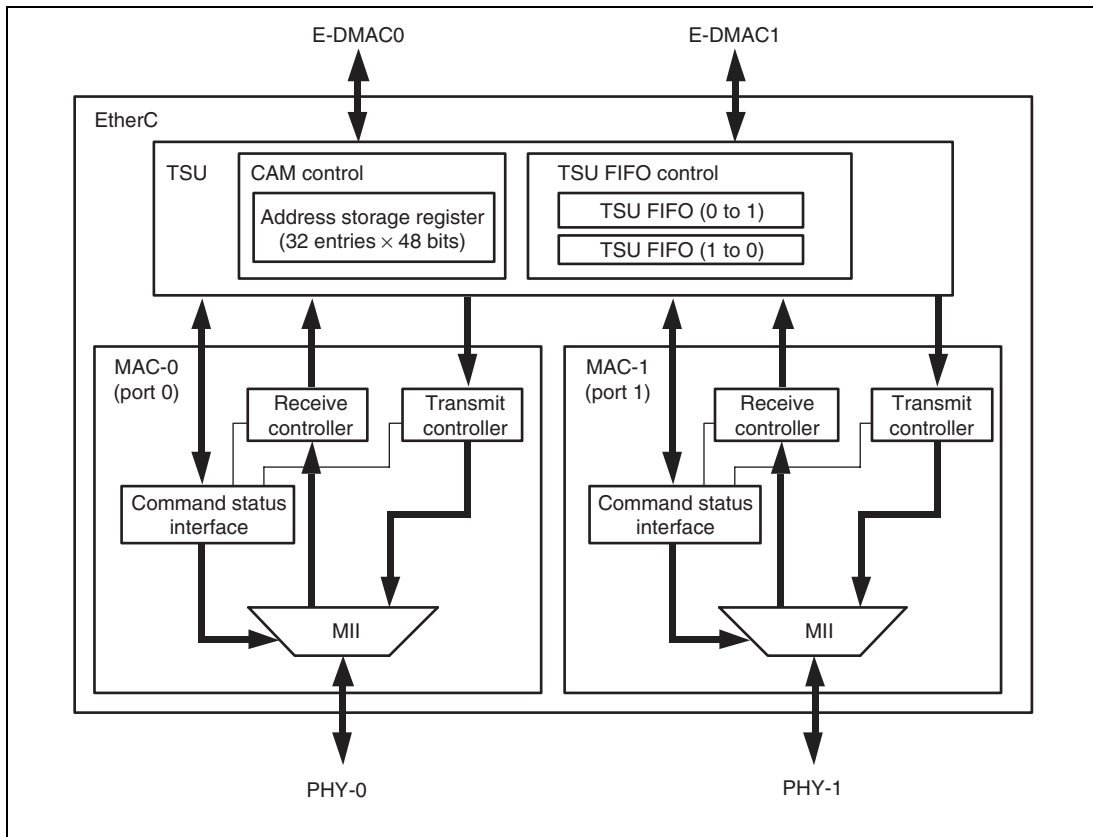
Figure 18.1 Configuration of EtherC
