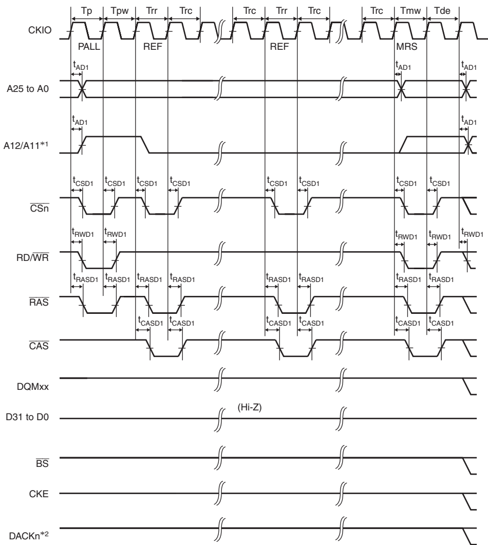
Figure 24.38 Synchronous DRAM Mode Register Write Timing (TRP = 2 Cycle)
