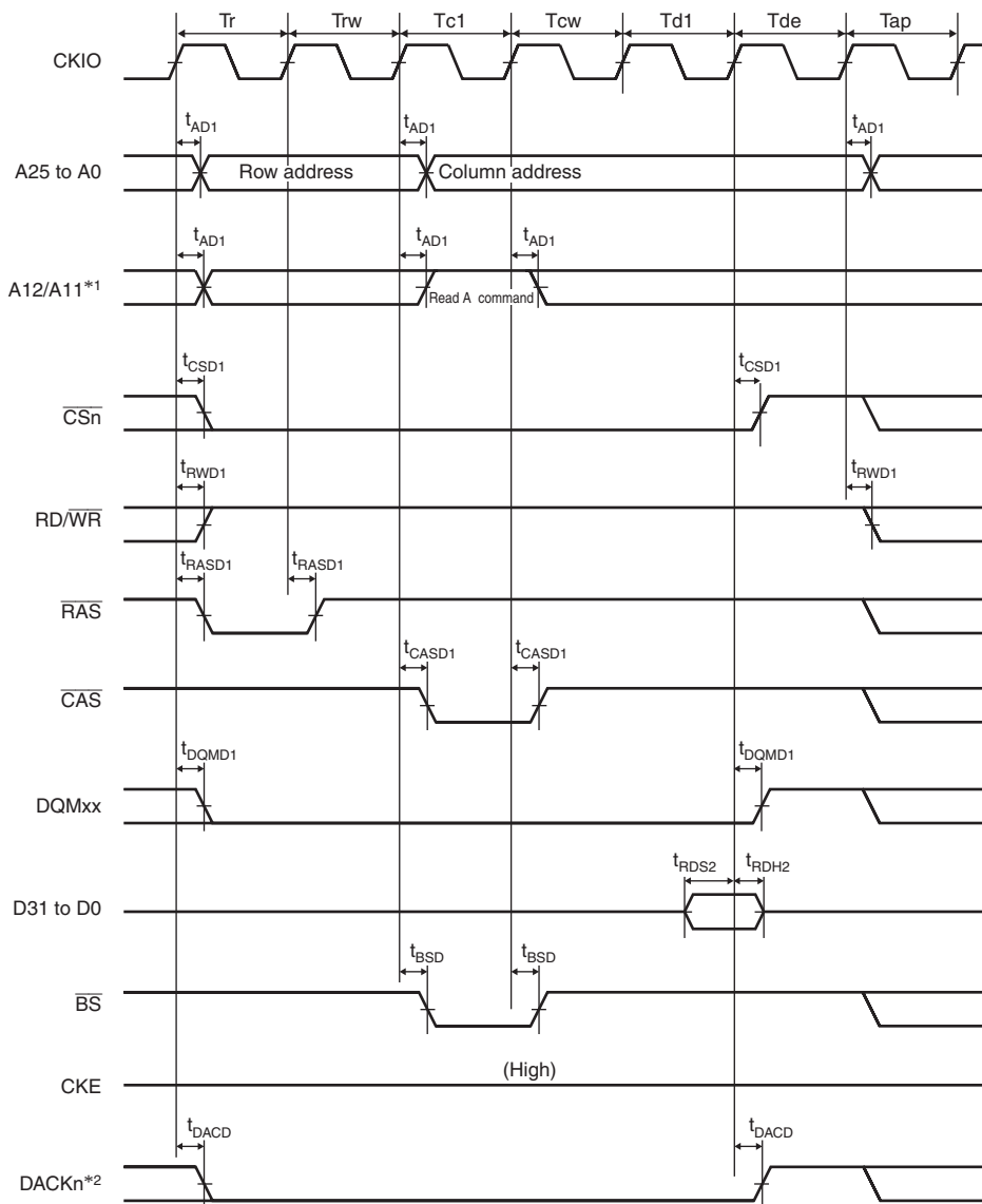
Figure 24.23 Synchronous DRAM Single Read Bus Cycle (Auto Precharge, CAS Latency = 2, TRCD = 2 Cycle, TRP = 2 Cycle)
