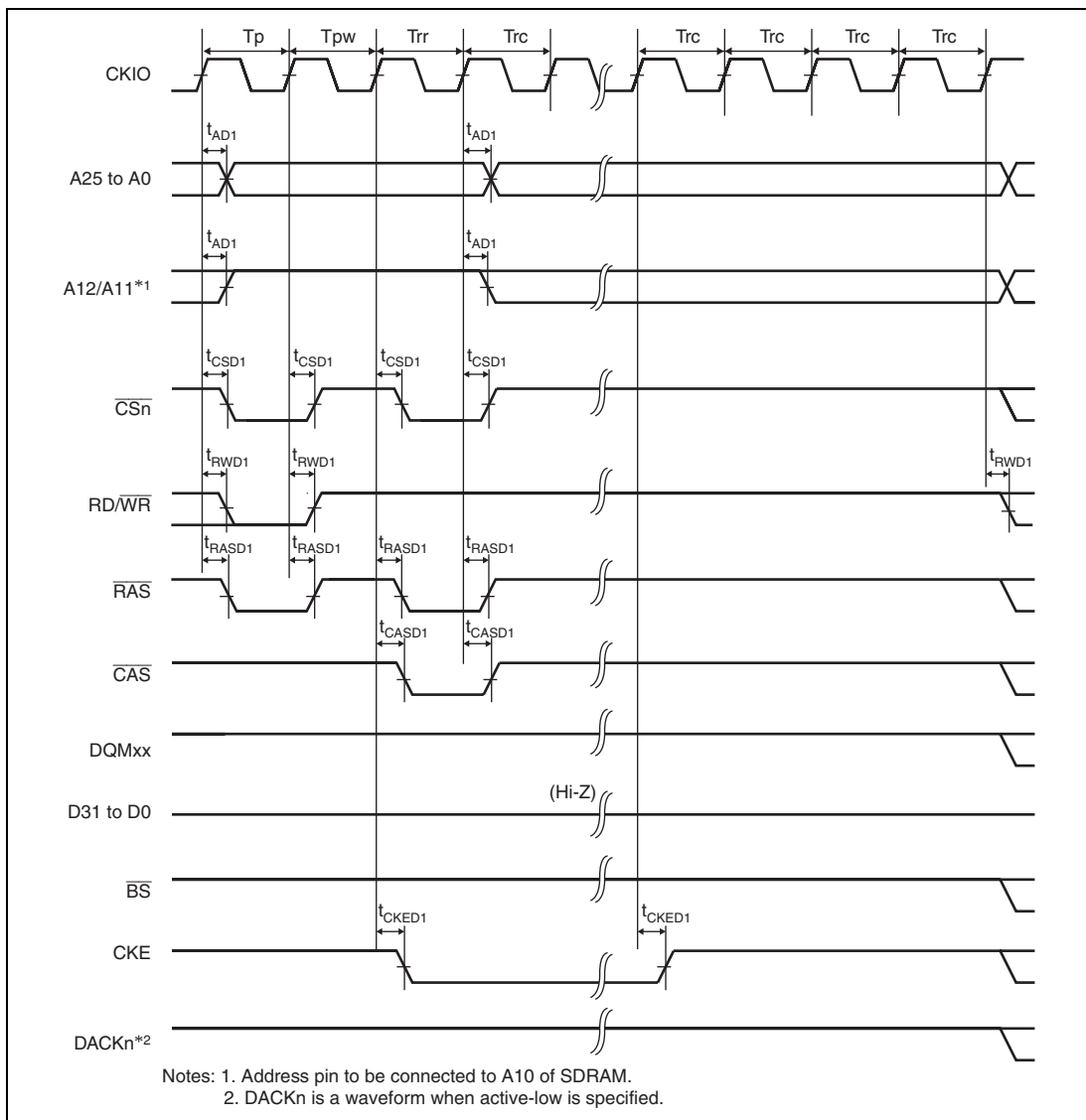
Figure 24.37 Synchronous DRAM Self-Refresh Timing (TRP = 2 Cycle)
