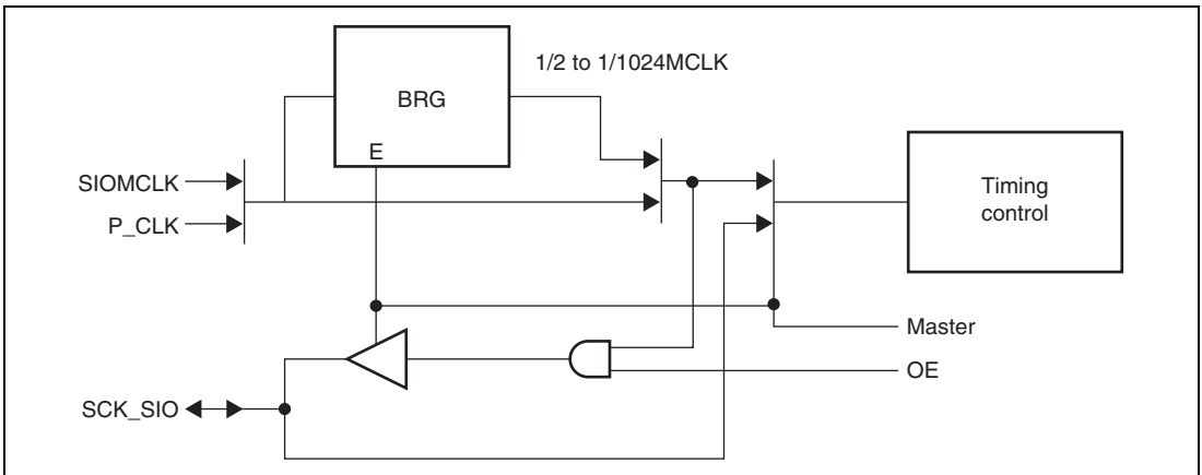
Figure 17.2 Serial Clock Supply
