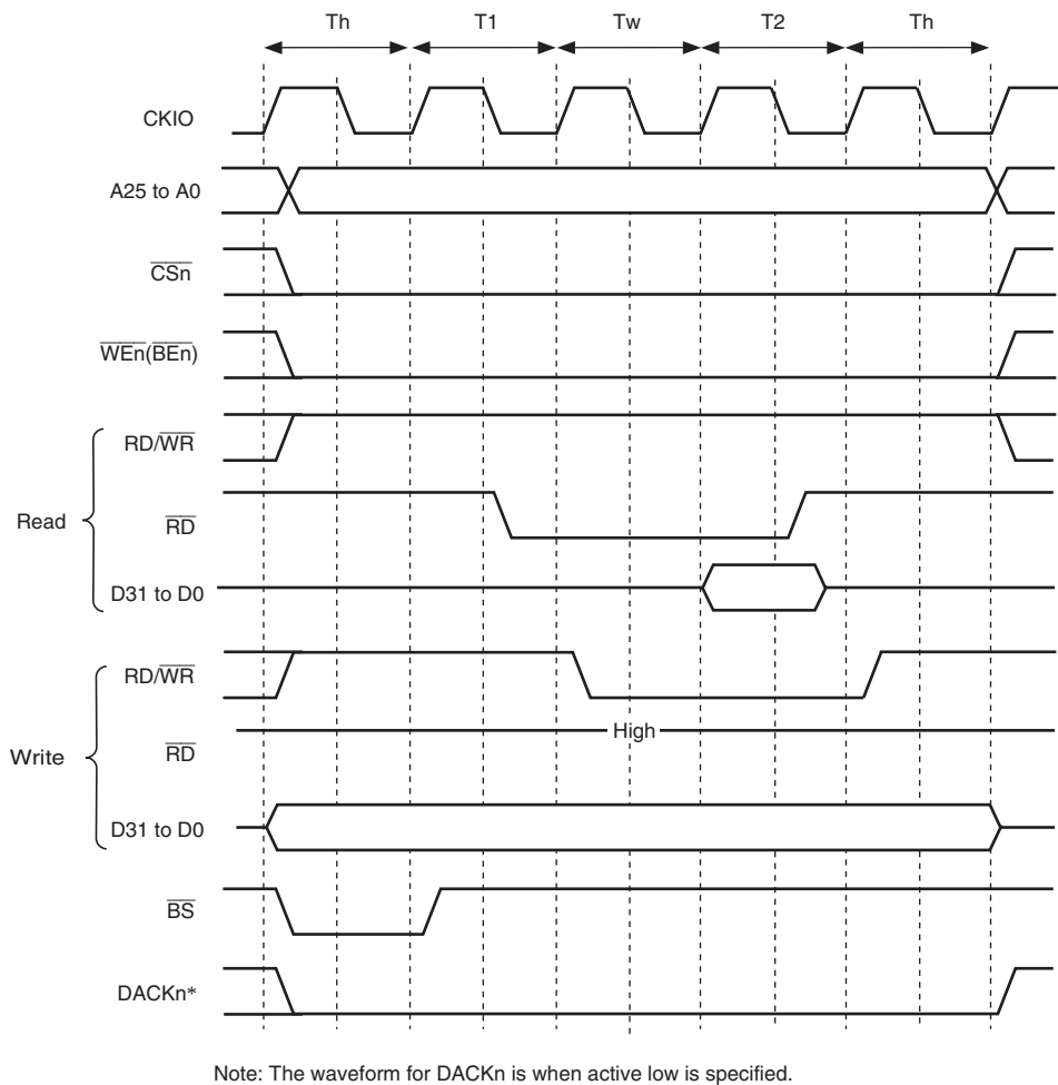
Figure 12.35 Wait Timing for Byte-Selection SRAM (BAS = 1) (Software Wait Only)
