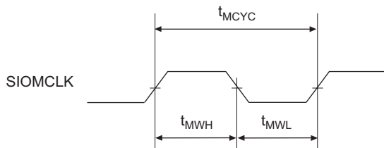
Figure 24.53 SIOMCLK Input Timing
