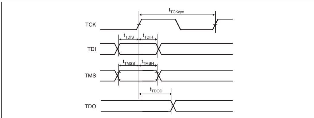
Figure 24.72 H-UDI Data Transfer Timing
