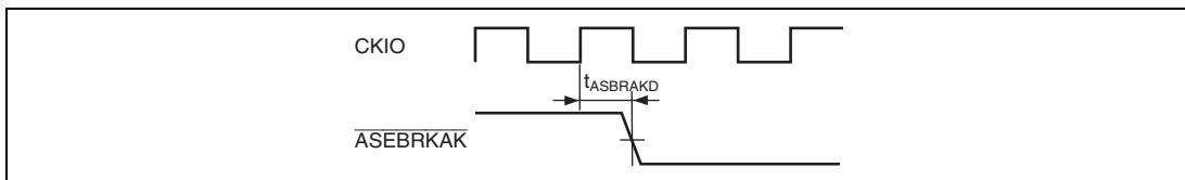
Figure 24.74 \overline{\text{ASEBRKAK}} Delay Time
