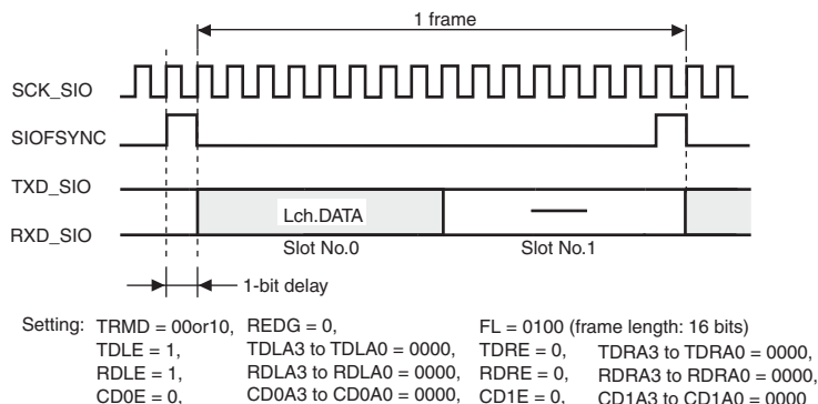
Figure 17.14 Transmission and Reception Timings (8-Bit Monaural Data (2))
