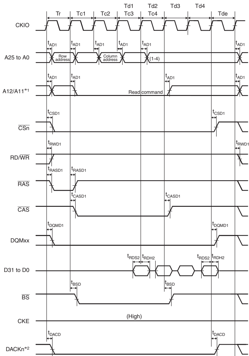
Figure 24.30 Synchronous DRAM Burst Read Bus Cycle (Single Read \times 4 ) (Bank Active Mode, ACTV + READ Commands, CAS Latency = 2, TRCD = 1 Cycle)
