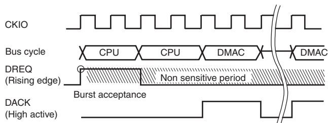
Figure 13.14 Example of DREQ Input Detection in Burst Mode Edge Detection
