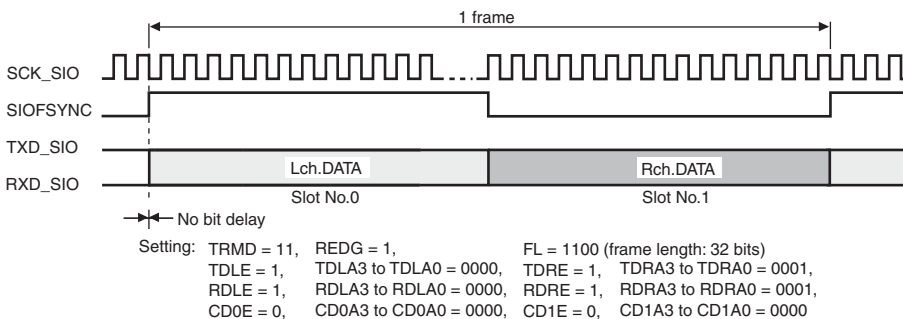
Figure 17.16 Transmission and Reception Timings (16-Bit Stereo Data (1))
