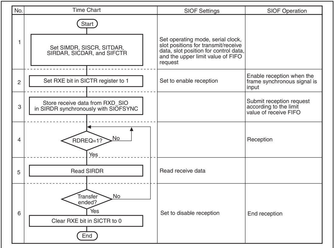
Figure 17.12 Example of Reception Operation in Slave Mode
