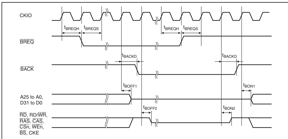
Figure 24.14 Bus Release Timing
