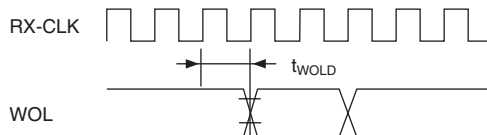
Figure 24.65 WOL Output Timing
