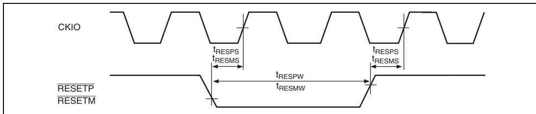
Figure 24.12 Reset Input Timing
