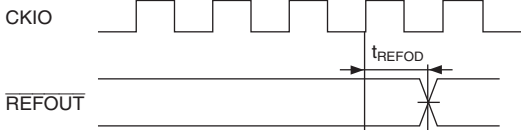
Figure 24.43 REFOUT Delay Time
