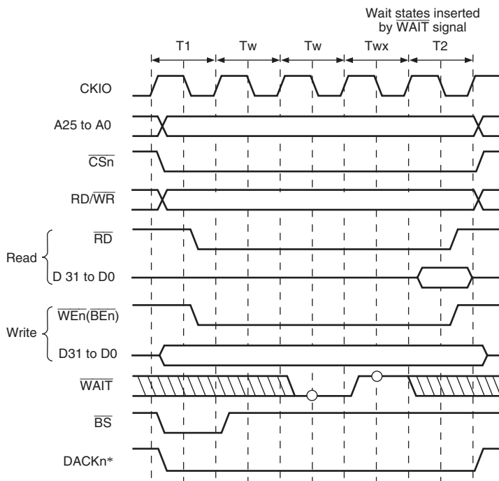
Figure 12.10 Wait State Timing for Normal Space Access (Wait State Insertion by \overline{WAIT} Signal)
