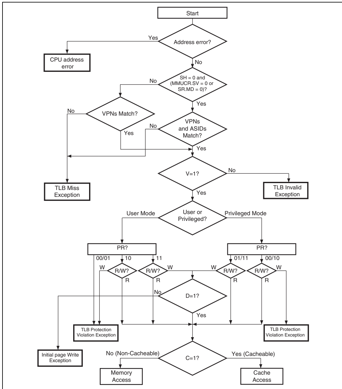
Figure 5.13 MMU Exception Generation Flowchart
