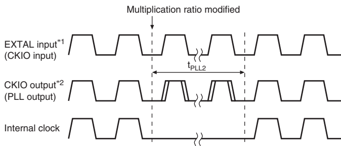
Figure 24.10 PLL Synchronization Settling Time by IRQ/IRL Interrupts
