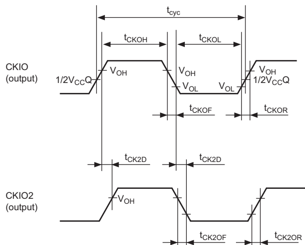
Figure 24.4 CKIO Clock Output Timing
