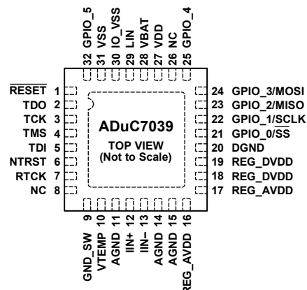
Figure 3. Pin Configuration
