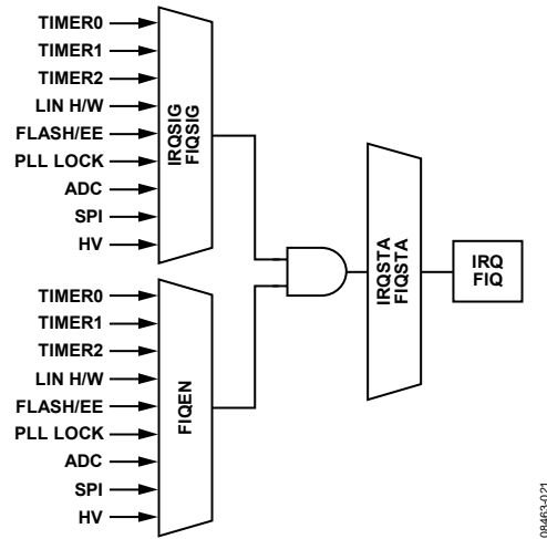
Figure 22. Interrupt Structure
