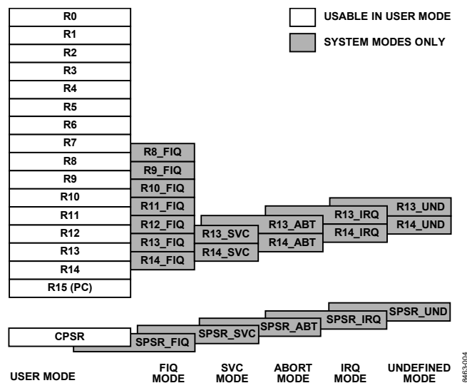
Figure 4. Register Organization
