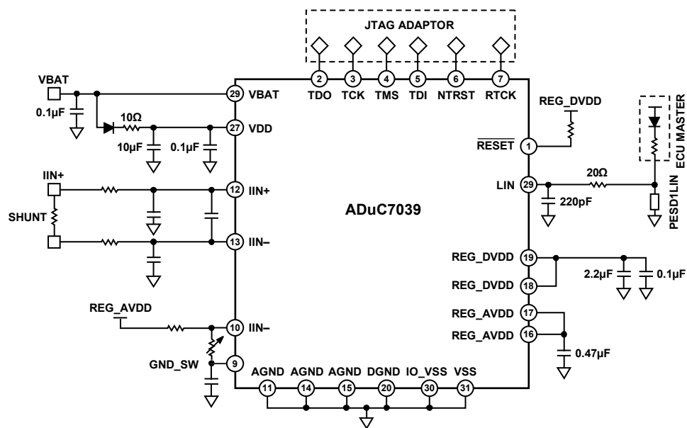
Figure 33. Recommended Schematic
