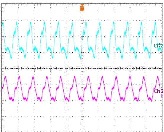
Output voltage ripple at nominal input voltage and max load current Top trace +12V, 10mV/div, Bottom trace -12V, 20mV/div, 2μs/div. Load cap: 10μF, tantalum capacitor and 1μF ceramic capacitor. Bandwidth: 20MHz.
